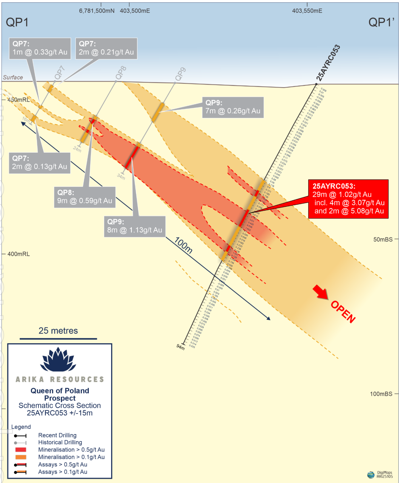
Figure 4: Schematic Cross-Section Line 2680mN (local grid) showing recent drilling results. Note the mineralised zone improving in thickness and grade down-dip from the shallow historical holes.
