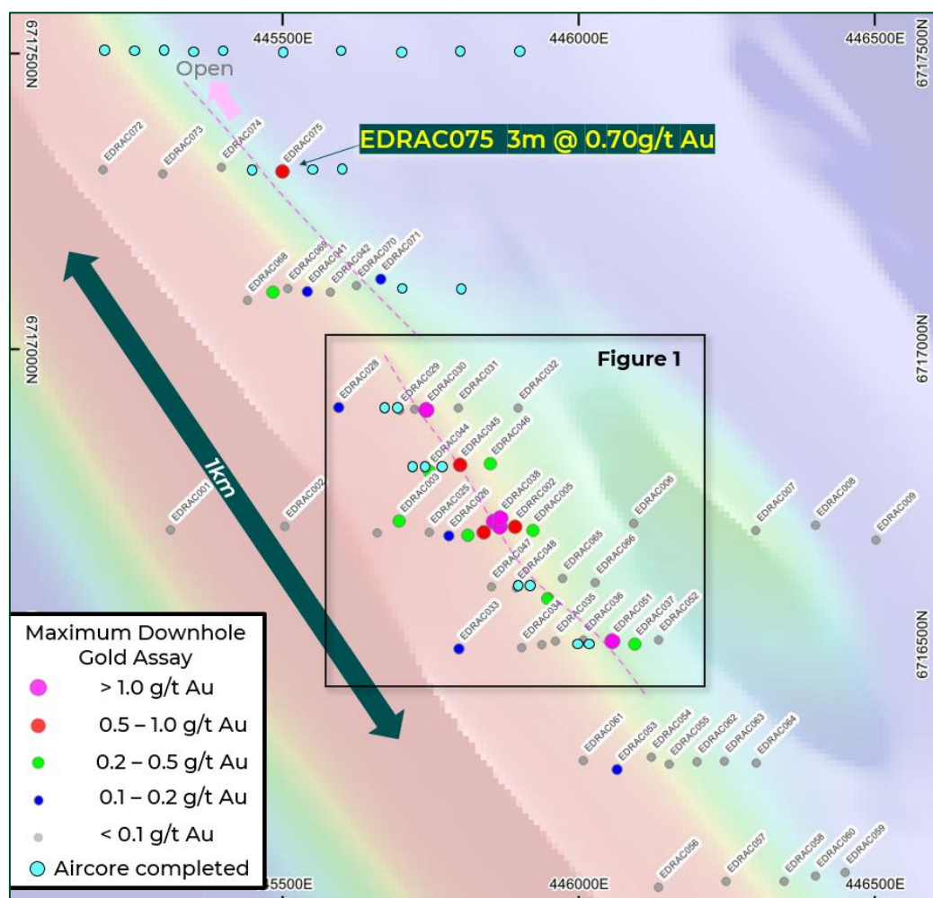
Figure 2: All aircore drilling at Edjudina Range and peak down-hole gold values 2 showing the location of recent aircore holes (light blue- assays pending). Refer to Figure 1 for inset details.
