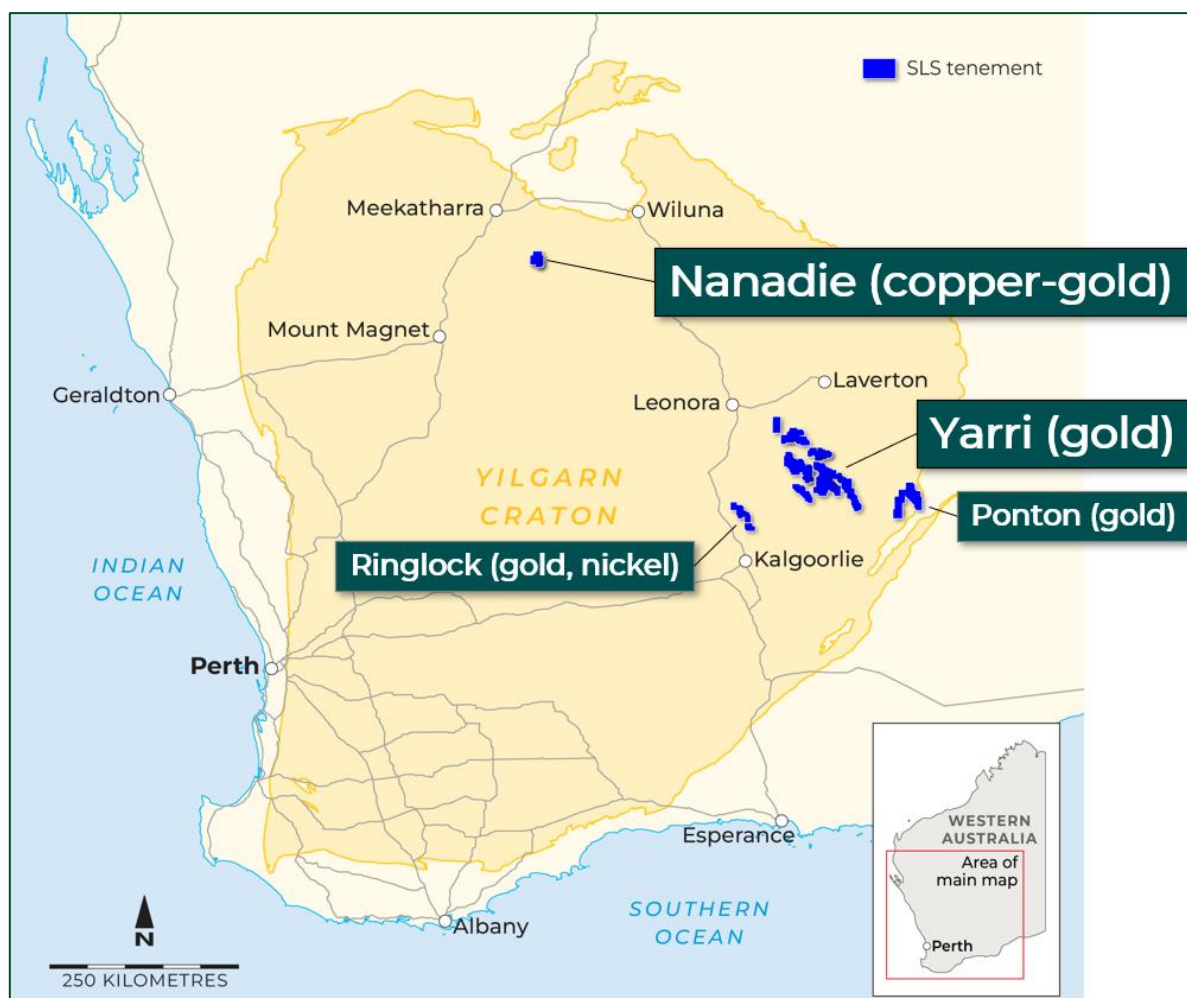
Figure 5: Location of Solstice's West Australian Projects.
