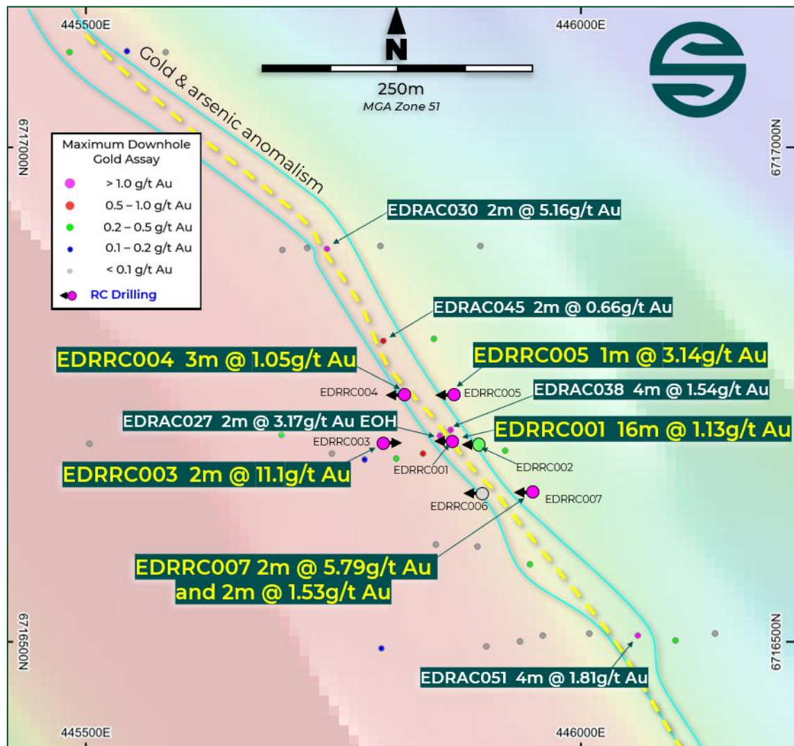
Figure 1: Central part of the Edjudina Range discovery with all RC and aircore drillholes coloured for peak down-hole gold values 2 , and significant intercepts following 1m resampling (text boxes), on aeromagnetic imagery. The interpreted trend of bedrock arsenic anomalism (below transported cover) is also shown.
