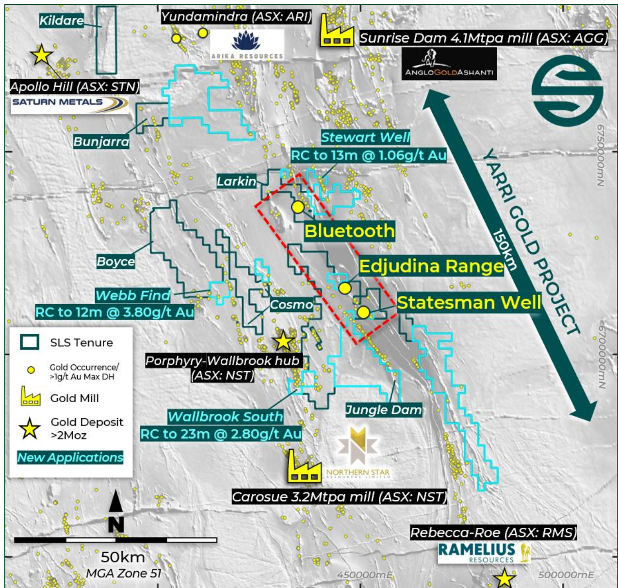
Figure 4: Solstice's >1,600km 2 Yarri Project tenement group on greyscale aeromagnetic image showing the location of key gold targets, new Exploration Licence applications 3 , and regional gold developments. Yellow dots are documented gold prospects and historical drillholes with >1g/t Au gold intercepts.
