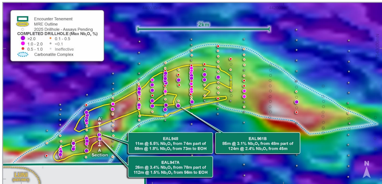
Figure 1 – Green Prospect - AEM - Layered Earth Inversion (LEI) DS55 showing arcuate conductive feature coincident with the outline of the weathered carbonatite complex (from geological logging) and MRE 2,3,4,5,6
