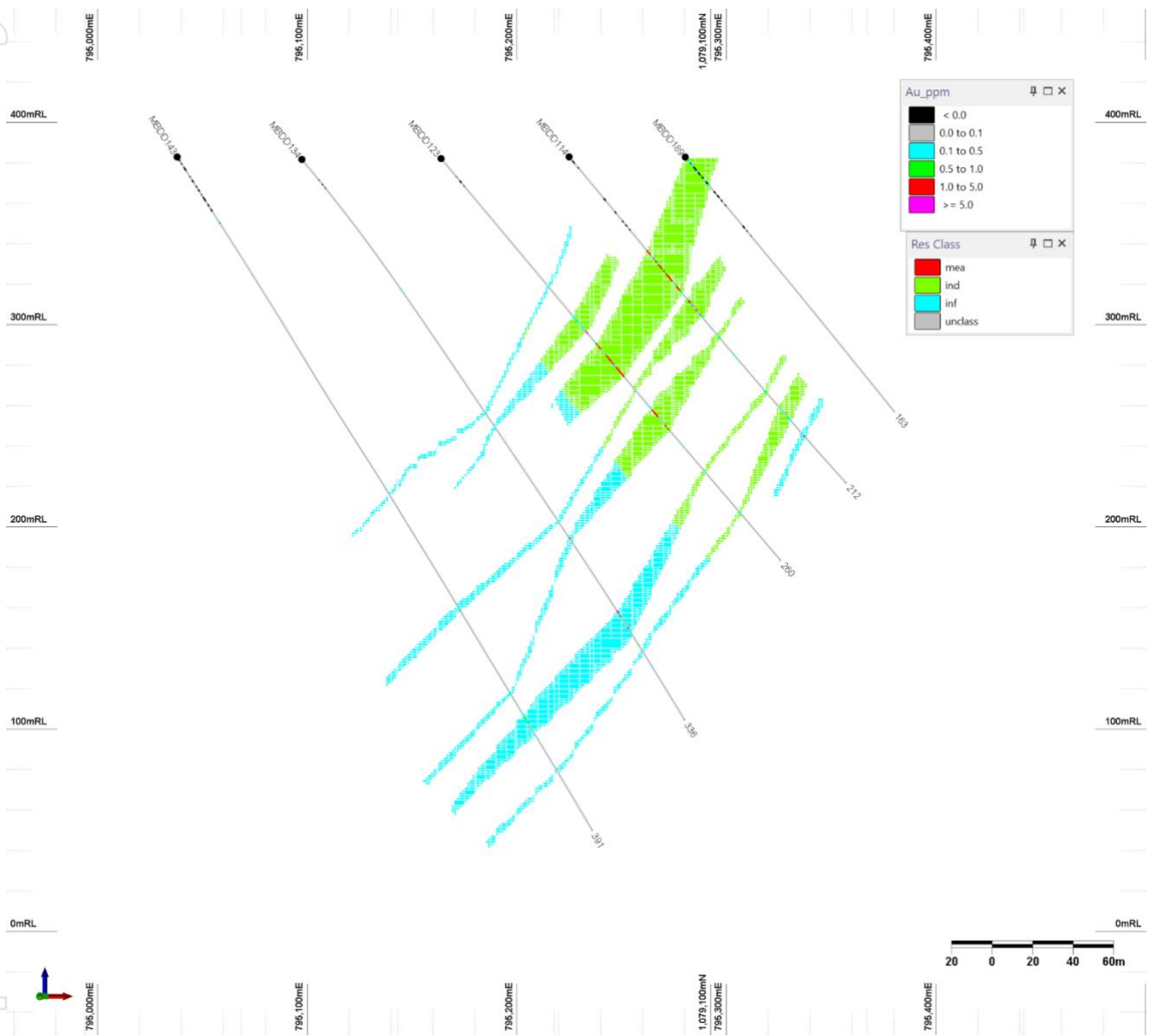
Figure 9: Example oblique cross section BMT3 showing resource classification and drill data (looking northeast +/-25m)
