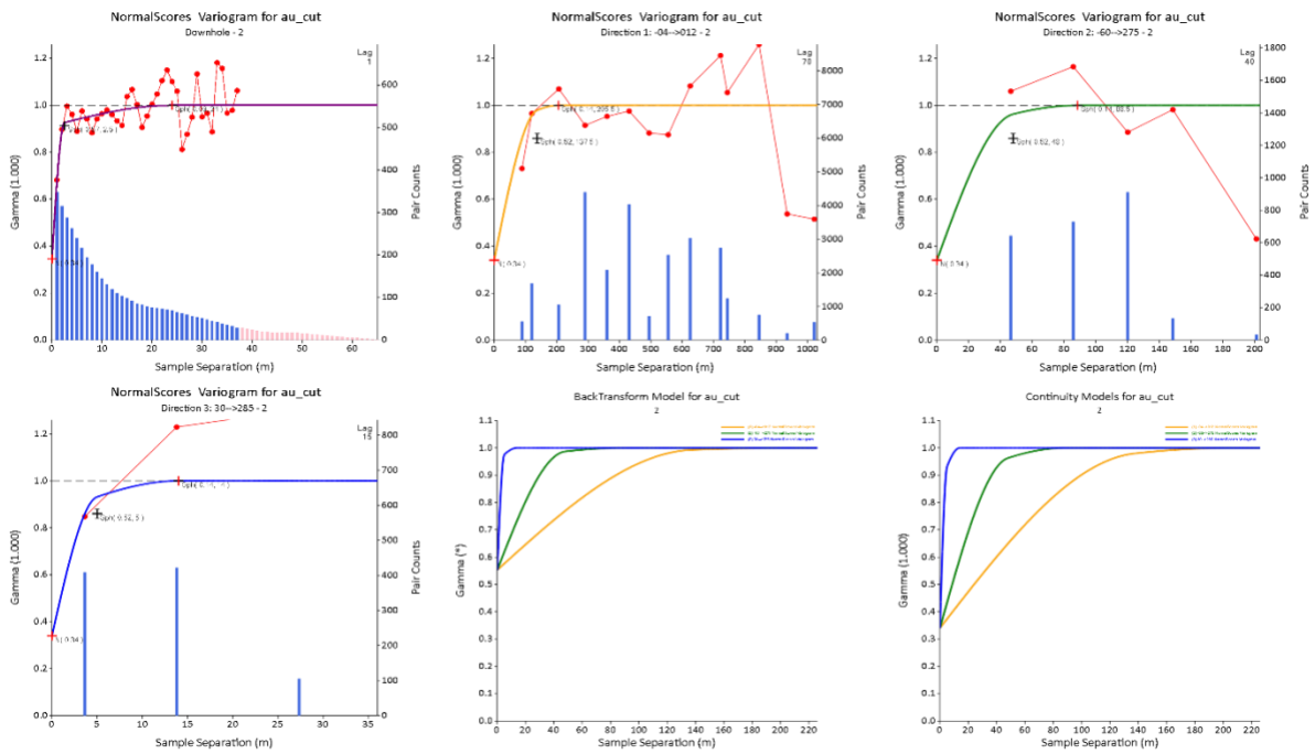
Figure 6: Experimental Variograms and fitted models BMT3 Object 2
