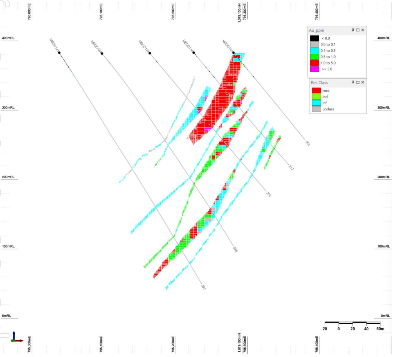
Figure 8: Example oblique cross section BMT3 showing estimated gold grades and drill data (looking northeast +/-25m)
