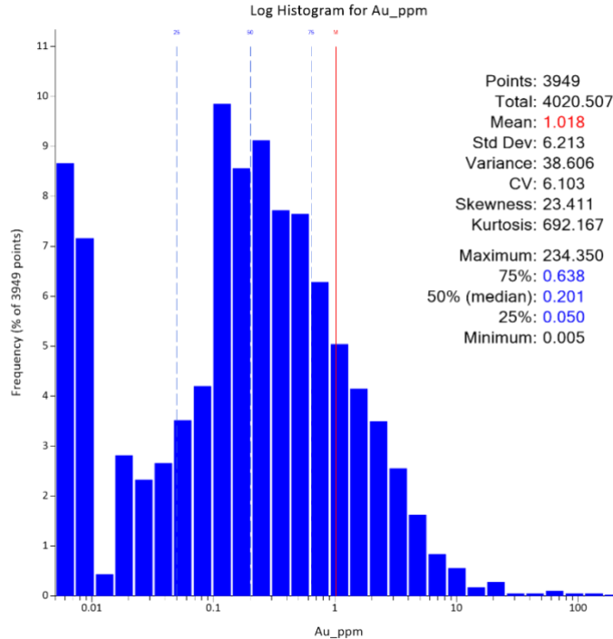
Figure 5: Log histogram for BMT3 composites
