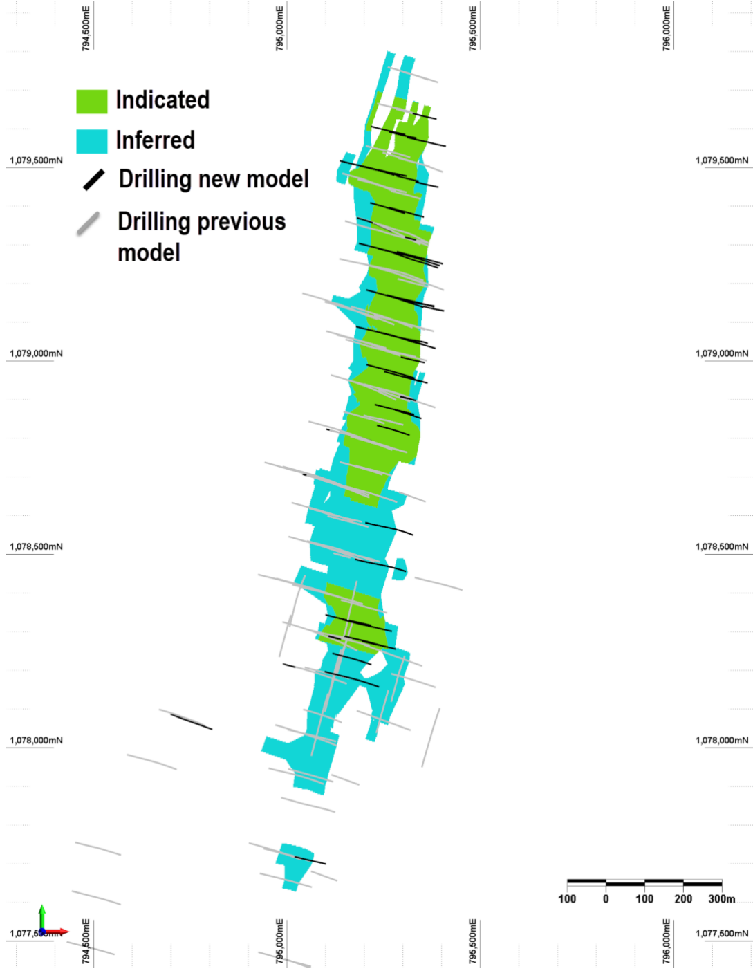
Figure 7: Plan view of BMT3 showing model classification (projected to surface) and informing drilling
