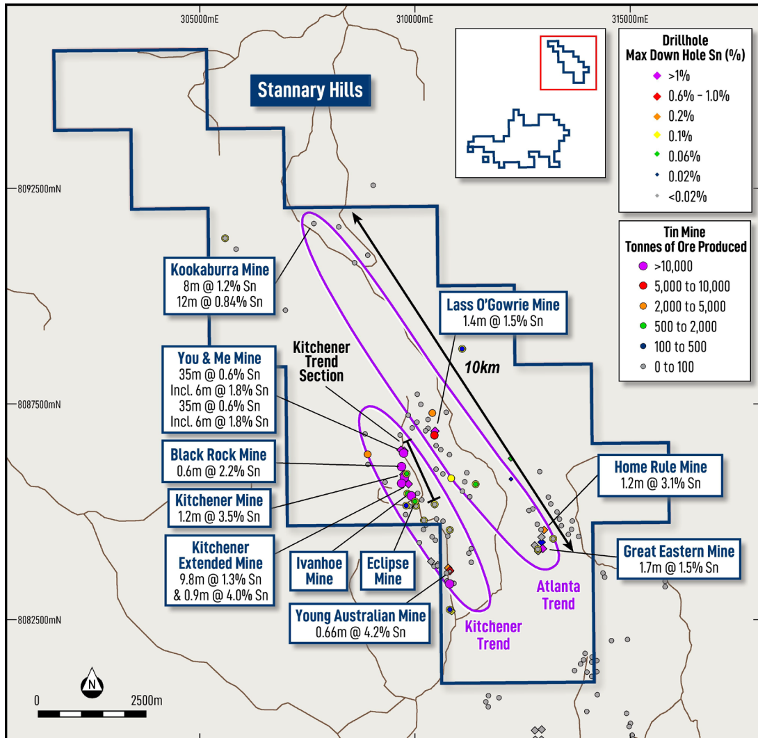
Figure 3: Plan of the Stannary Hills Project showing the extensive mineralisation in drilling and historical mines along the Kitchener and Atlanta Trends, also see Figure 4.
