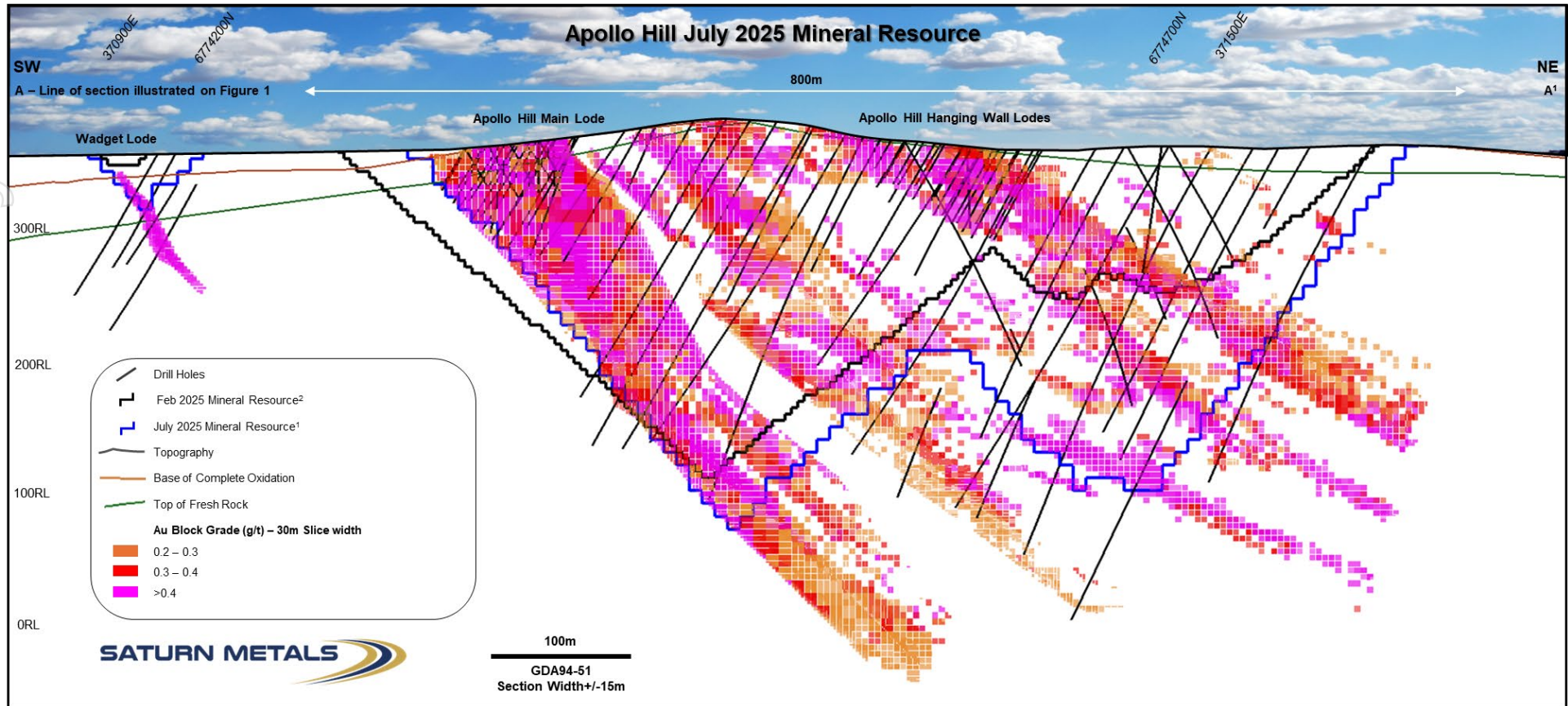
Figure 2 – Oblique block model cross-section (South West – North East, A-A 1 on Figure 1 3D diagram) ± 15 m showing gold grade and block location.
