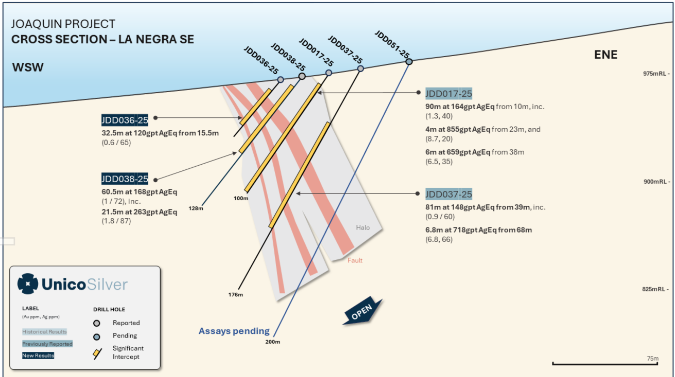
Figure 4: La Negra SE, JDD036-25 and JDD038-25 Cross Section
