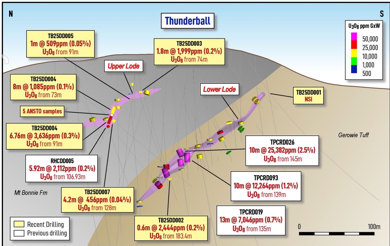
Figure 3 – Long section A-A', clipped to 40m, looking East at Thunderball. Mineralisation envelope can be seen in pink, with intercepts from this programme shown as yellow text boxes and historic as white text boxes. The lower lode sits in the Gerowie Tuff just below the contact with the Mt Bonnie Formation whilst the upper lode is within a more tuffaceous unit of the Mt Bonnie formation.
