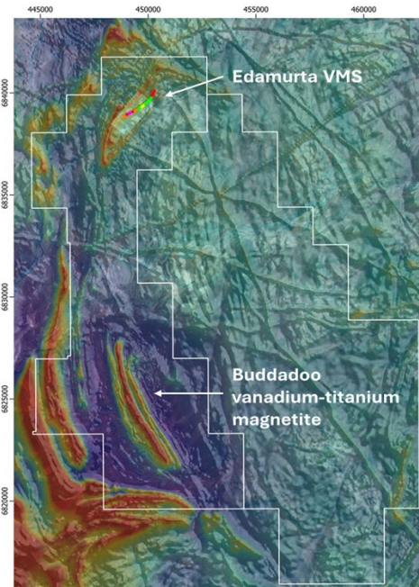
Figure 7. Regional magnetic with Edamurta MLEM plates overlay
