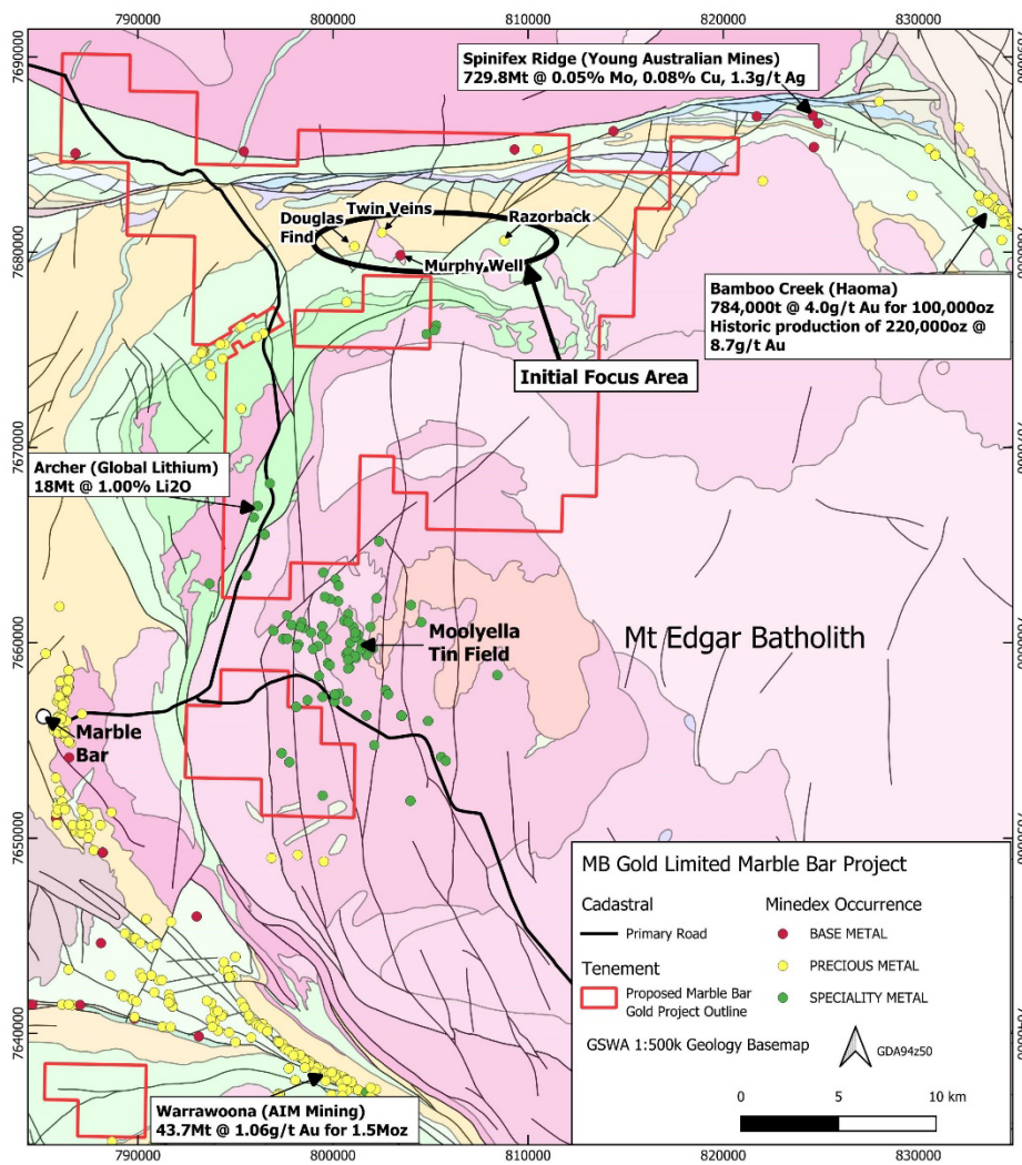
Figure 1: Marble Bar Gold Project and prospect location map on the 1:500,000 GSWA interpreted bedrock geology basemap, including third-party projects and Mineral Resources 6,7,8 .
