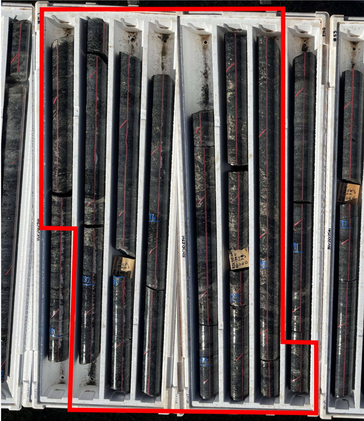
Figure 2. Core photographs of the interval of significant sulphides annotated with the visual chalcopyrite percentage.
