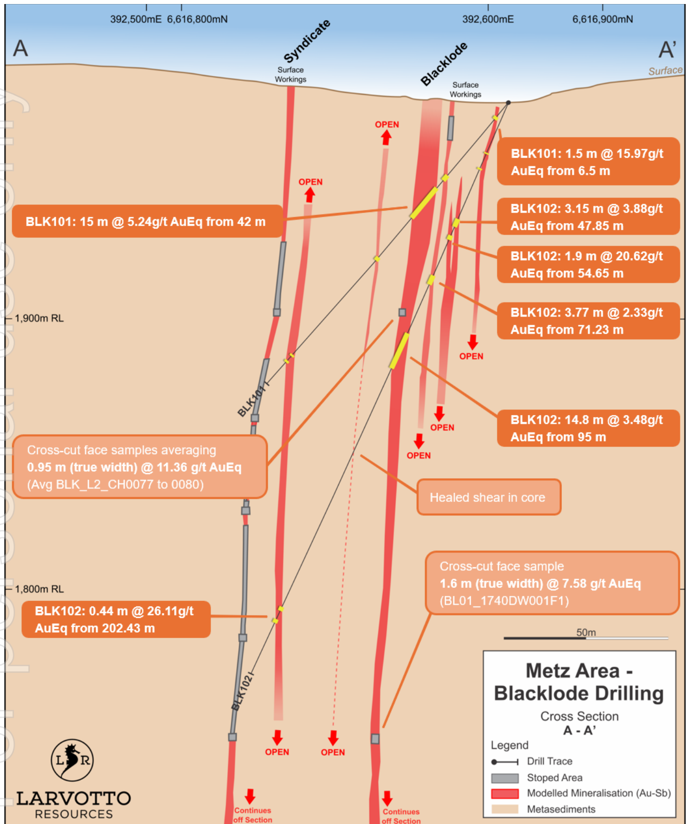
Figure 3 Blacklode Cross-section A-A' (top 300m)
