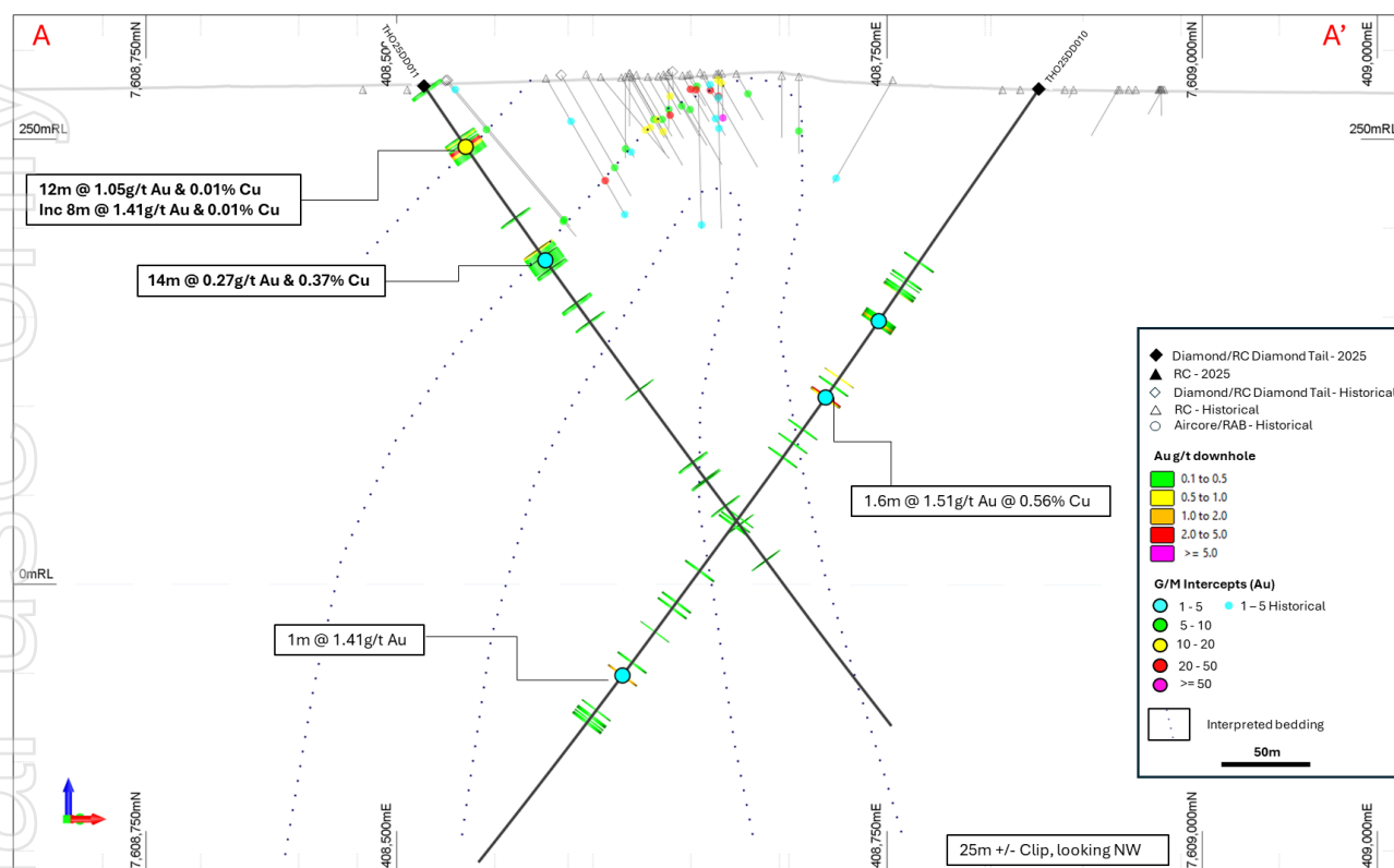
Figure 153: Thomsons oblique section showing drilling results and historic drilling
