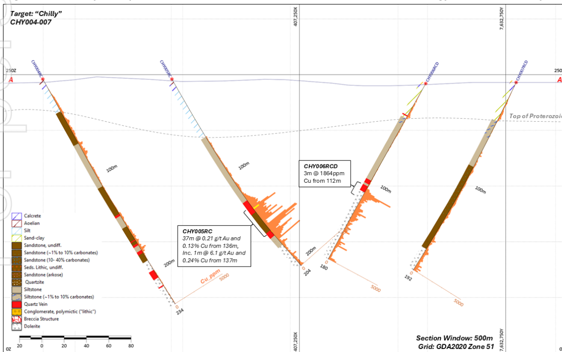
Figure 19: Chilly oblique section orientation 050° – CHY004 – 007; Lithology, Au & Cu assays
