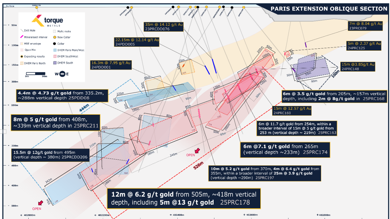
Figure 2 Paris deposit oblique view, DHEM indicating extensions in multiple directions
