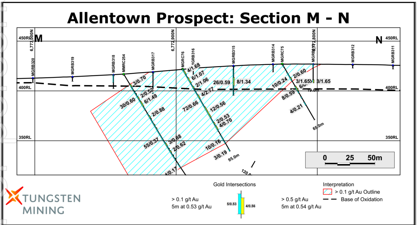
Figure 10. Section M-N showing broad zones of anomalous gold located 250 metres north of the Allentown Prospect.
