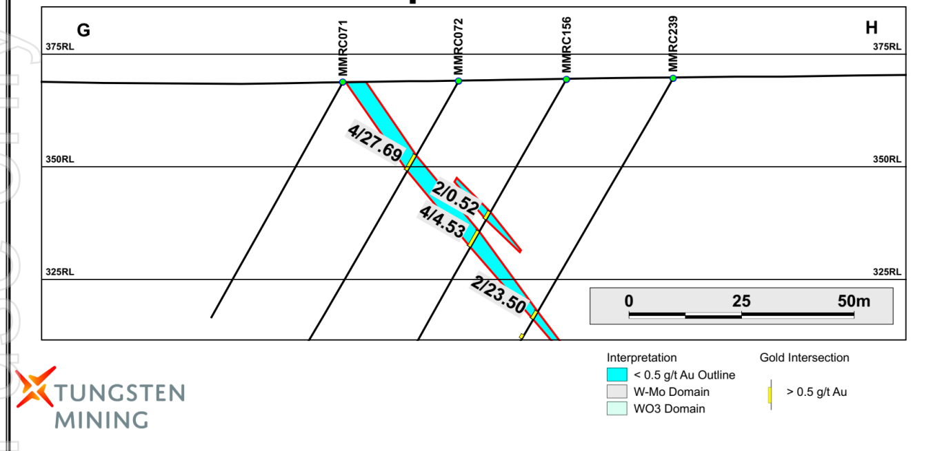
Figure 6. Section G-H showing high-grade gold mineralisation at the Monza Prospect.
