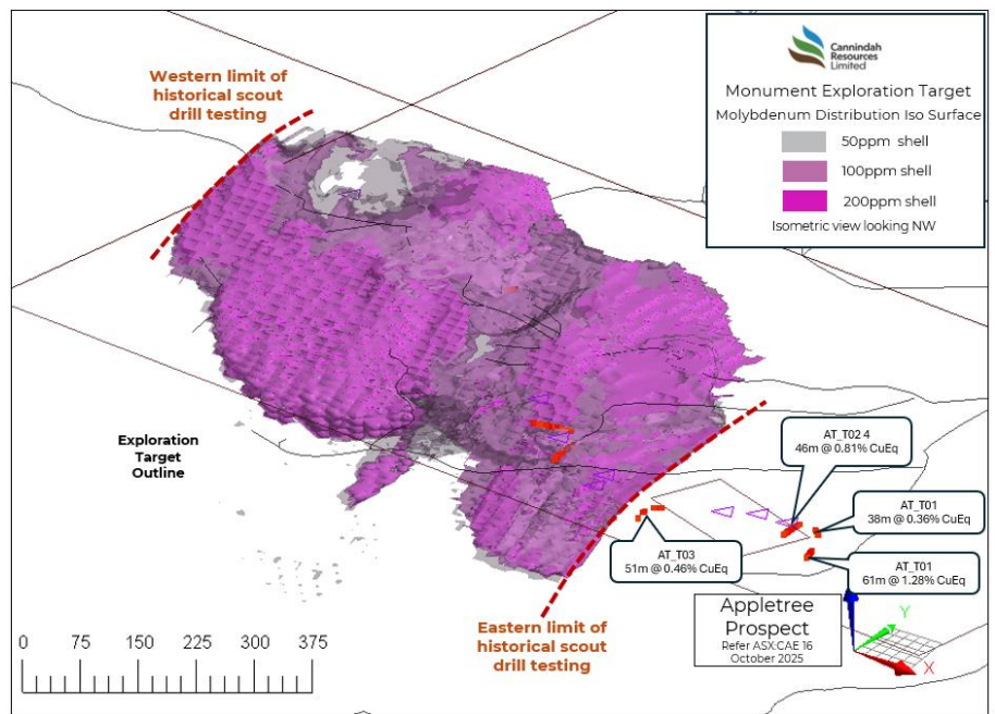
Figure 5: Distribution of the modelled Mo isosurfaces at the Monument Exploration Target within the Southern Target. Note the large area of +200ppm Mo. (isometric view looking down to NW)
