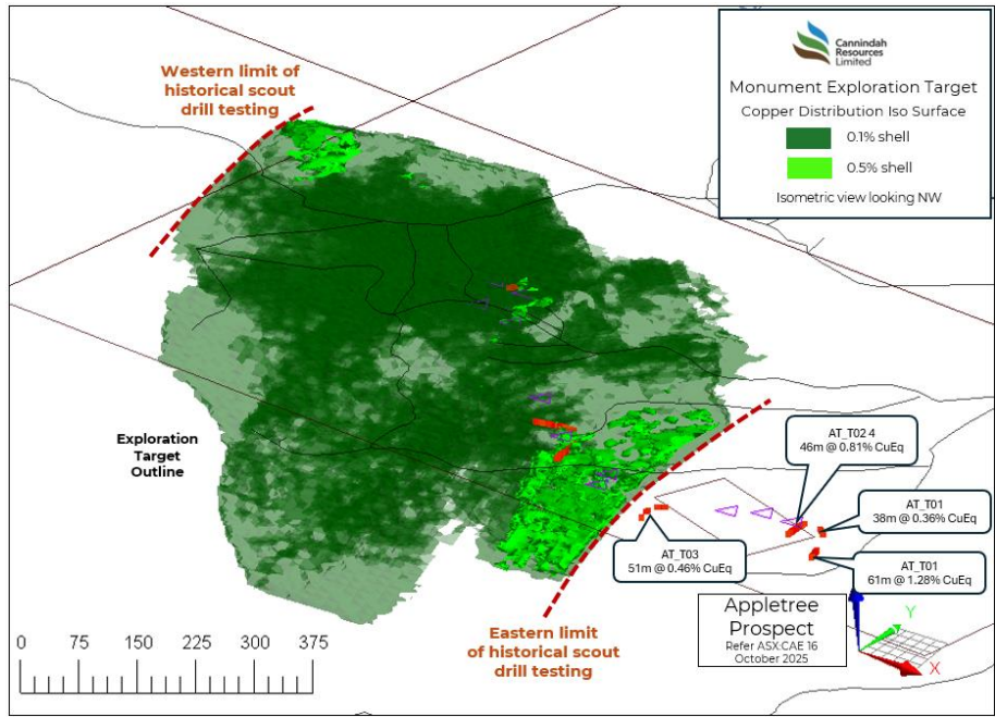
Figure 4: Distribution of the modelled Cu isosurfaces at the Monument Exploration Target within the Southern Target. Note the two (2) zones of +0.5% Cu. (isometric view looking down to NW)
