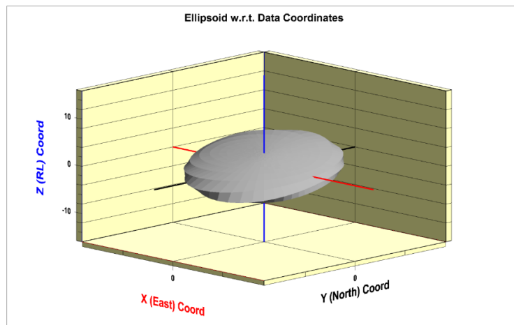
Figure 7 3D Variogram Model for the Monument Deposit
