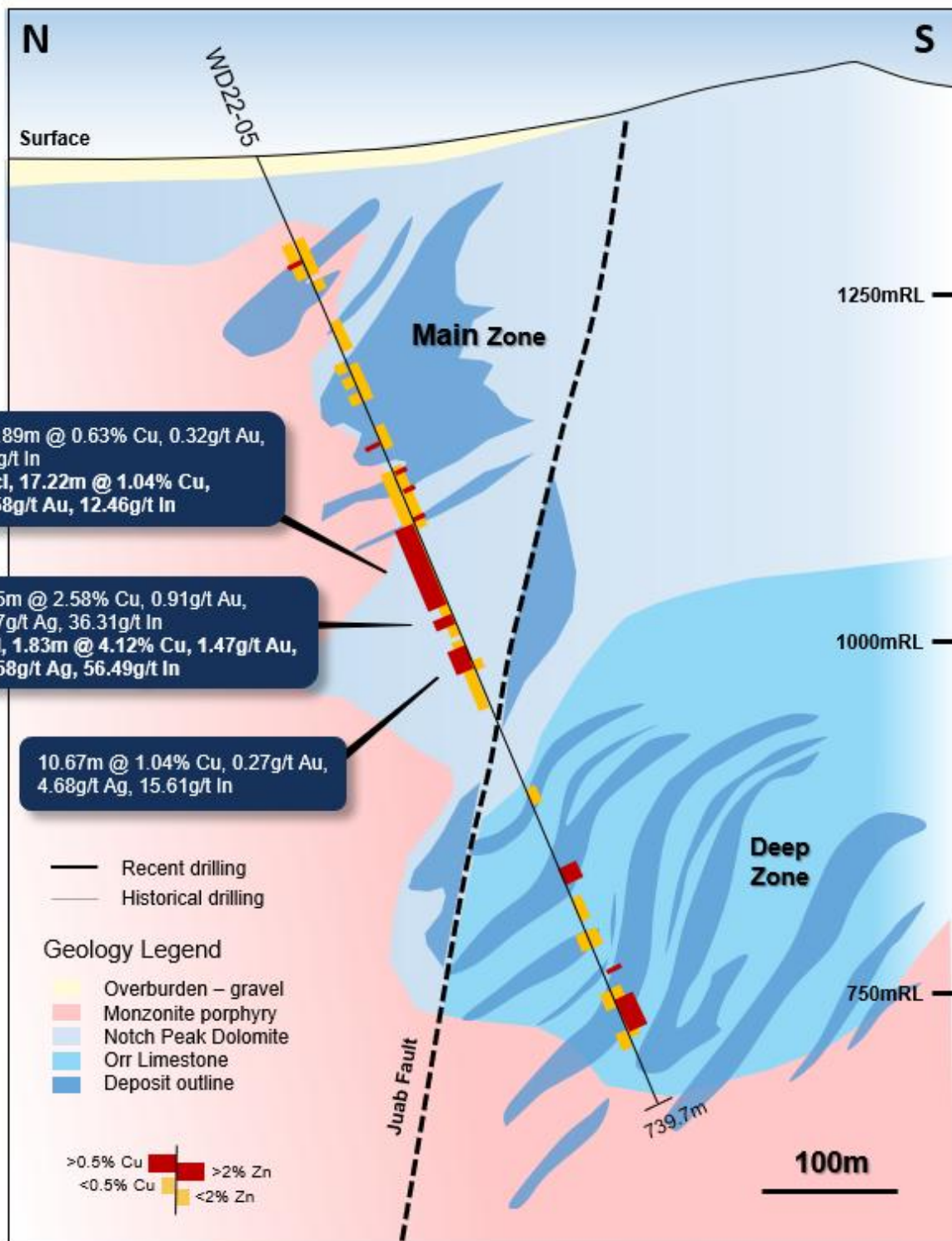
Figure 5: Schematic geological section of the West Desert Deposit at 288810E looking east showing an example of the intersections of copper-gold dominant mineralisation located outside of the current resource envelope (darker blue).
