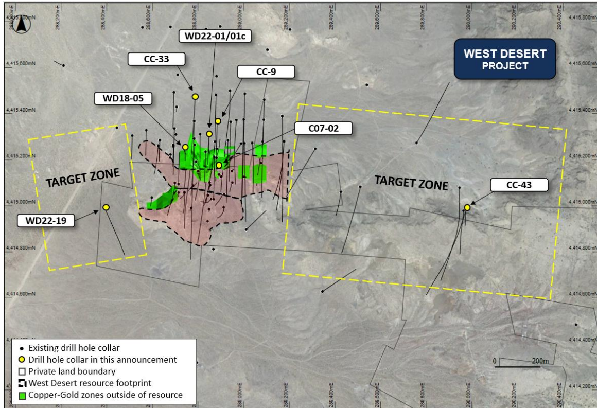
Figure 4: Plan view of the West Desert Deposit area overlaying topography.
