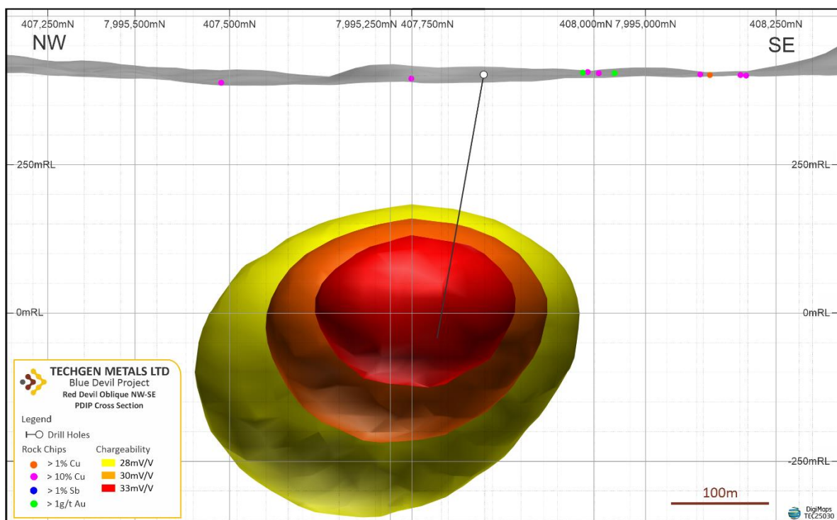
Figure 1: Red Devil 3D IP inversion model with surface rock chips shown.
