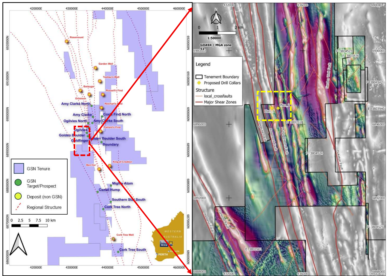
Figure 4 - Left: Tenure map of Great Southern Mining’s Duketon Gold Project showing key prospects, including the Ogilvies prospect within the Golden Boulder target area. Right: Map of the Golden Boulder area underlain by magnetic imagery (1VD TMI RTP) showing interpreted structures and the location of the two proposed EIS co-funded diamond drillholes.
