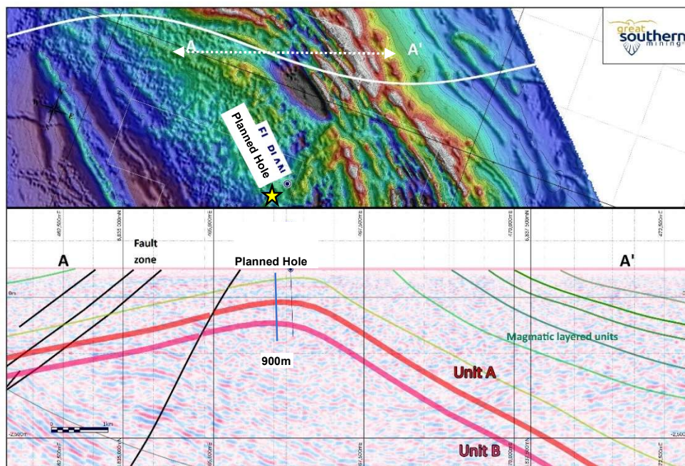
Figure 13 - Top - Magnetic imagery of the Diorite Hill Complex showing planned hole location (yellow star) and the location of the Geoscience Australia seismic line (curved white line). Bottom – Section line A-A’ showing seismic interpretation with target dense reflector horizons Unit A (red) and Unit B (pink) and the planned 900m drill hole (drill hole projected north onto the section).
