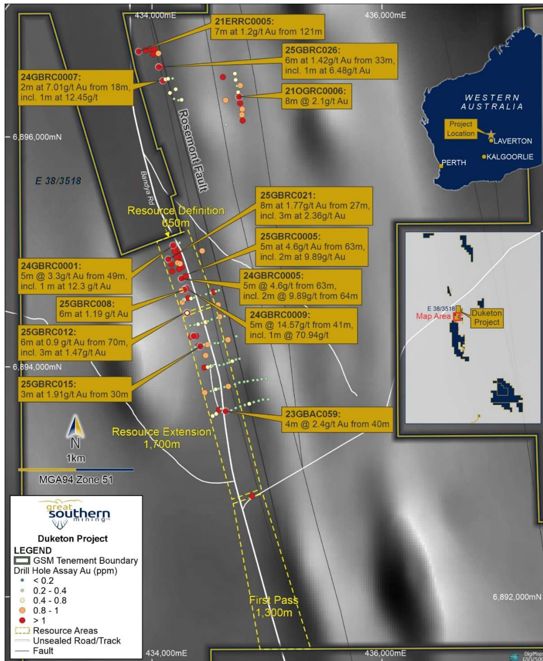
Figure 3 – Map of the Golden Boulder prospect area showing target areas for the current RC drilling program and selected intercepts from previous GSN drilling programs.
