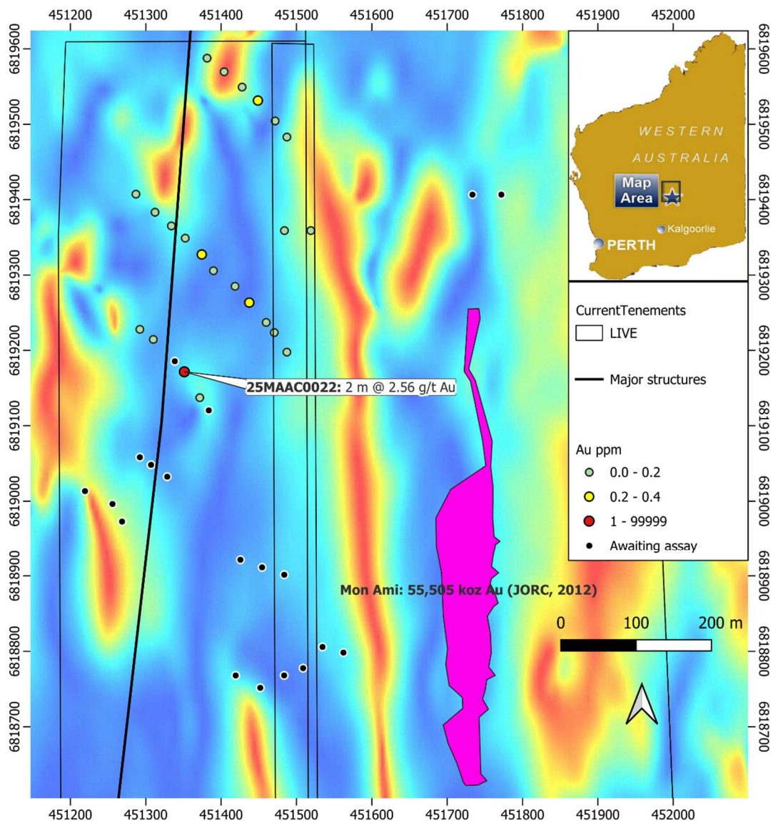
Figure 10 – Location map showing the location of recently completed aircore drilling at the Mon Ami Project, targeting a surface geochemical gold anomaly showing intercepts from assays received and those outstanding.
