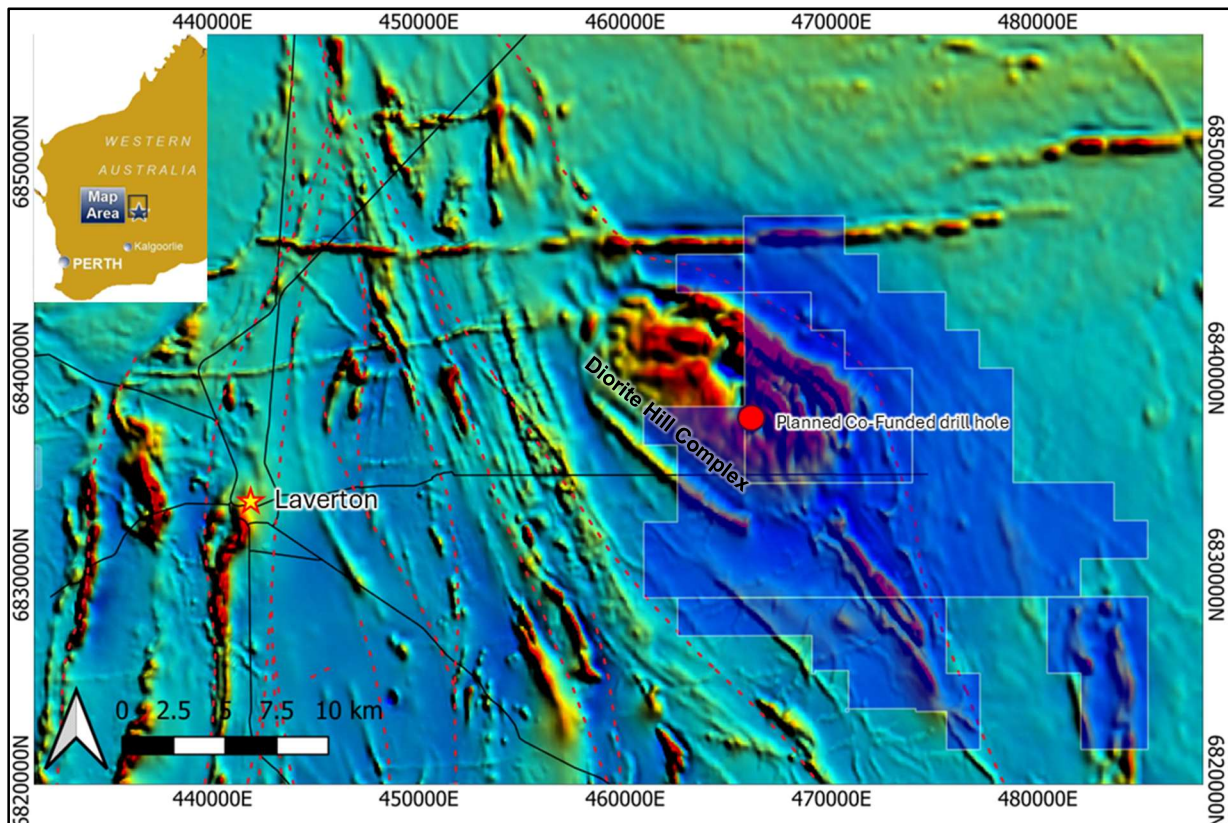
Figure 11 - Location of the East Laverton Project over regional aeromagnetic imagery. The Diorite Hill layered intrusive complex is evident as a large circular magnetic high (red colour) in the northwest of GSN's tenure (blue polygons).
