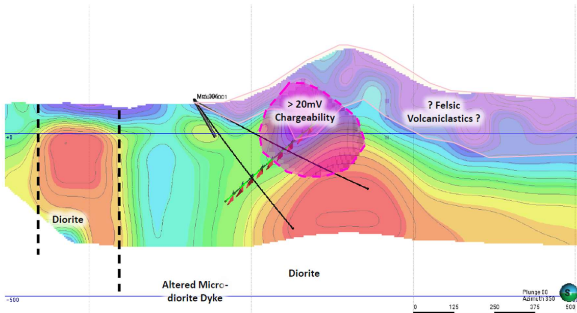
Figure 9 – Cross section of the Mt Dillon target showing proposed drill hole traces planned to intercept a >20mV chargeable IP anomaly.
