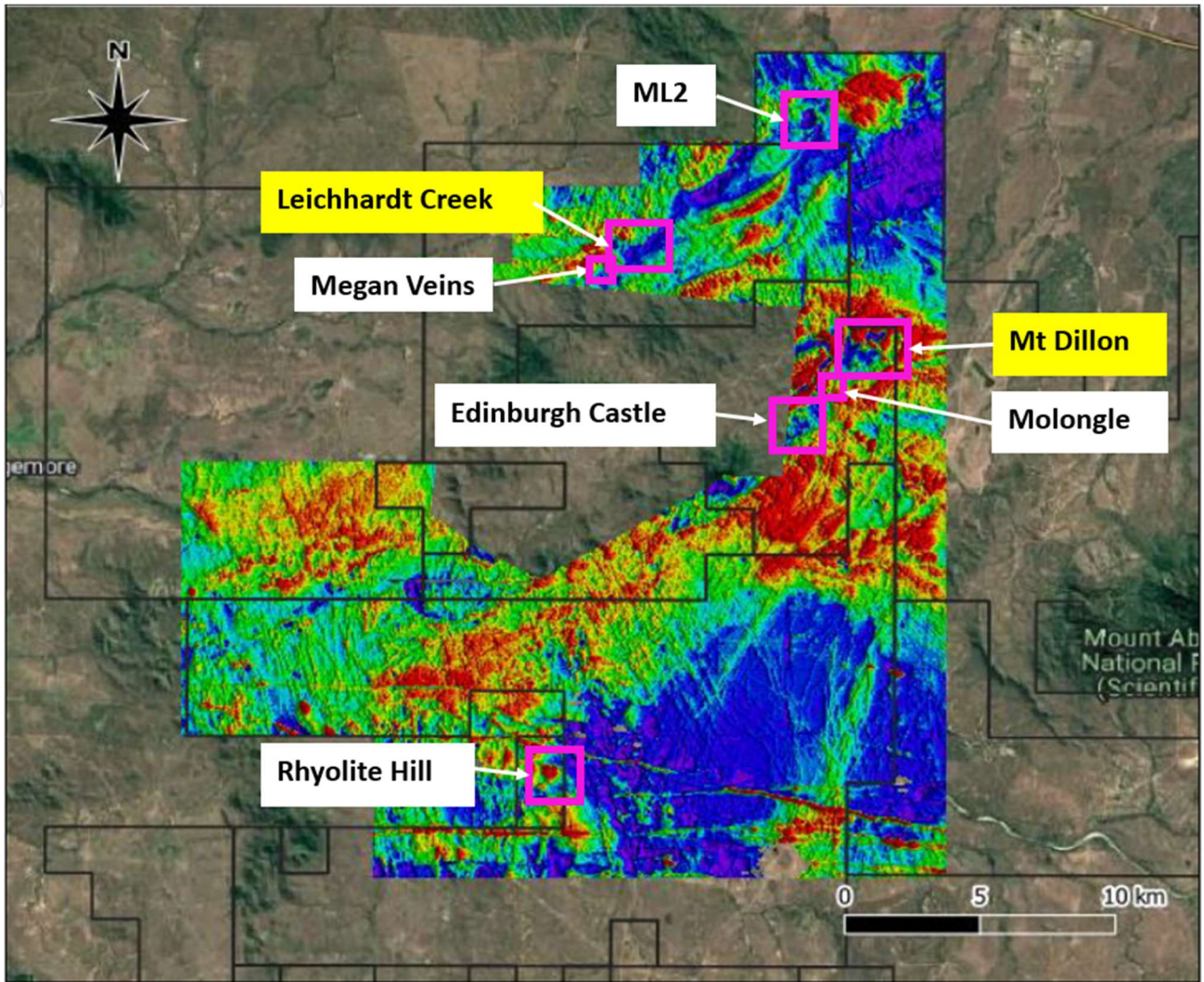
Figure 7 - Map of northern licences at Edinburgh Park, over magnetic imagery, showing high priority target areas including Megan Veins and Molongle.
