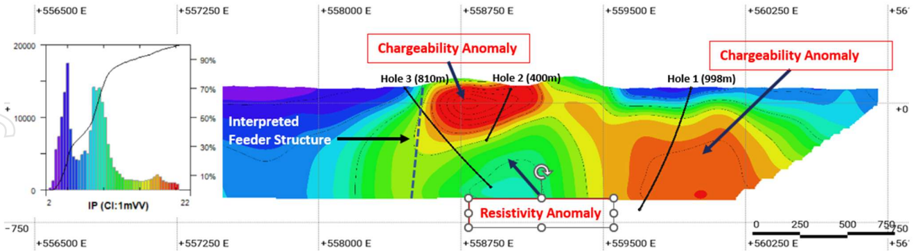
Figure 6 - South looking cross-section showing Leichhardt Creek completed holes 1 to 3, showing IP chargeability/resistivity anomalies and an interpreted mineralisation feeder structure.
