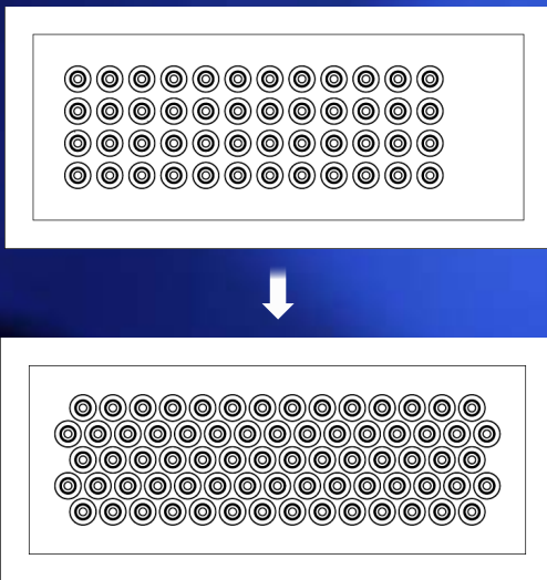
Figure 4 – Diagram showing the packing of cells in same size module from 48 to 72 cells
