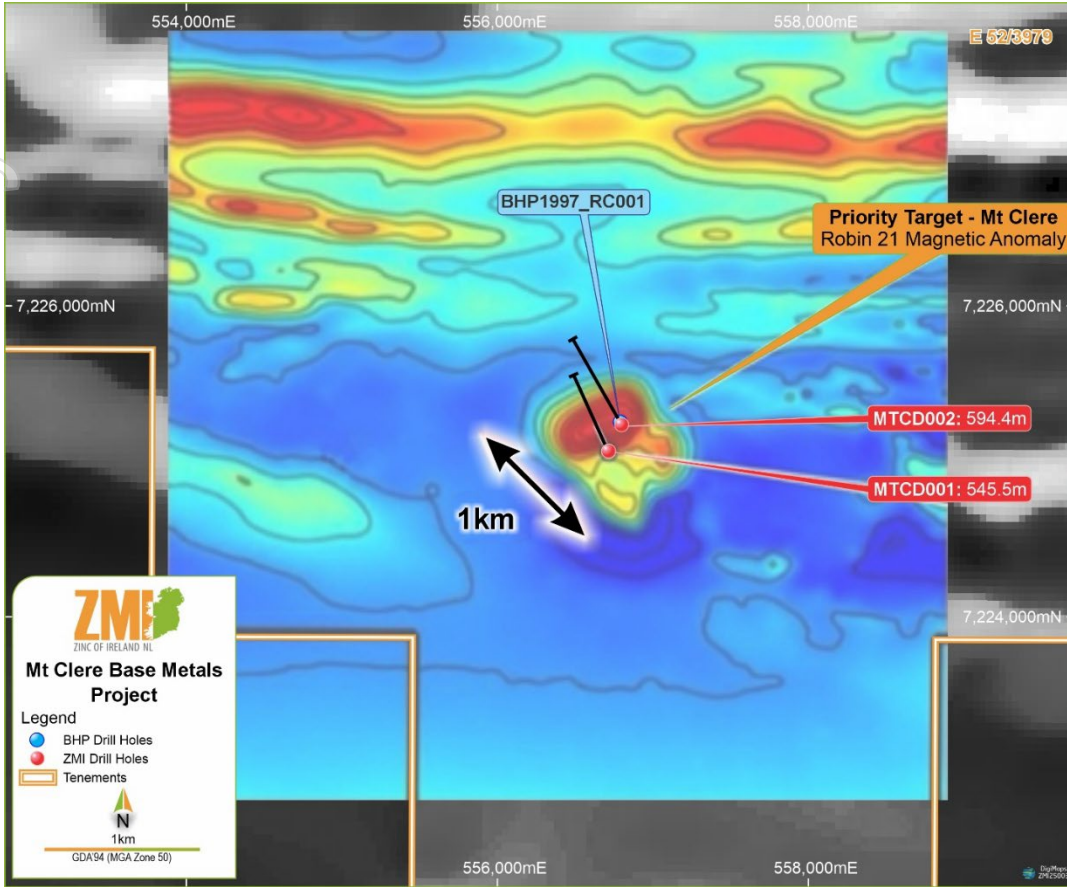
Figure 4. Drill Hole location plan BHP RC Hole (abandoned), MTCD 001 and MTCD 002 and Mt Clere magnetic anomaly (TMIRTP-IVD anomaly overlying greyscale image).
