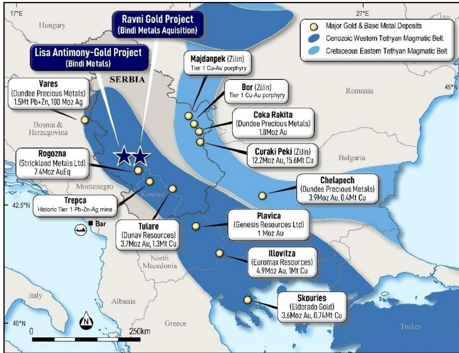
Figure 1: Ragni Project Location within the Tethyan Magmatic Belts well-endowed with large gold and base metals deposits.
