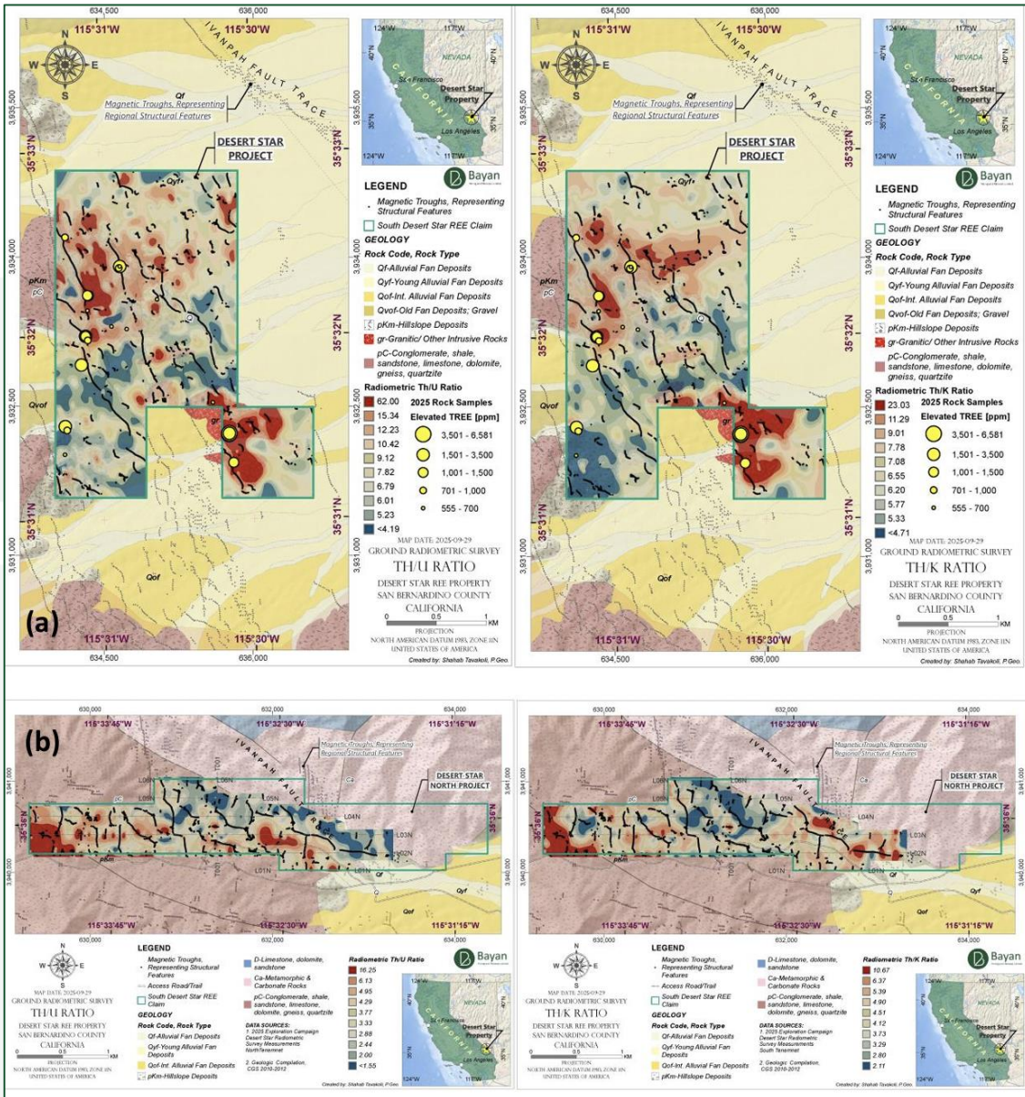
Figure 3: Radiometric Th/U and Th/K ratios (a) Desert Star South and (b) Desert Star North, representing relative radioelement abundance Th and U across the Desert Star Projects. Negative extrema in the Tilt Derivative (TDR) indicate probable NW trending faults and structural controls
