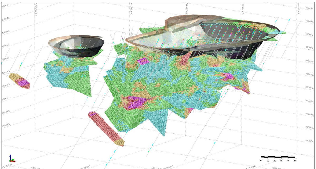
Figure 18: Toedter 3D view looking down to the north-west showing drill holes, mined open pits, and OK block model coloured by Au (g/t)
