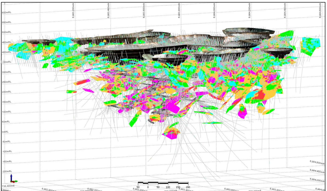
Figure 4: Swan/Swift 3D view looking down to the north-west showing drill holes, mined open pits, underground workings and OK block model coloured by Au (g/t)
