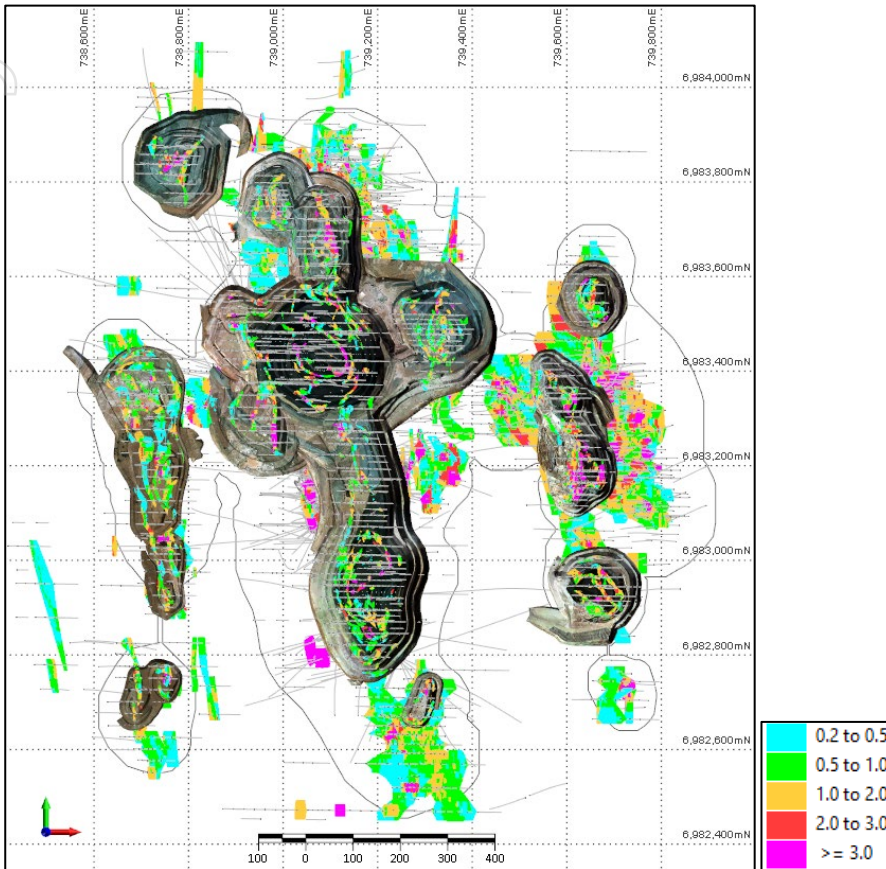
Figure 3: Swan/Swift drill hole plan showing mined open pits, OK resource block model coloured by Au (g/t) and A$4,500 optimised pit shell (grey outline)
