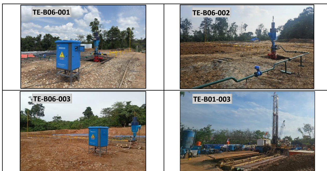
Dewatering and Drilling activities at Tanjung Enim Early Gas Sale well sites
