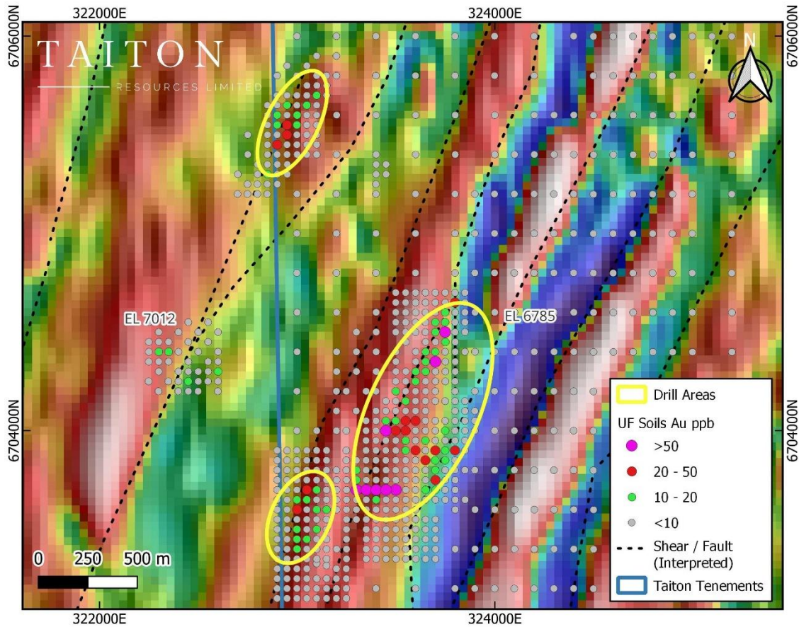
Figure 2. Challenger West Area 1 UF soil results underlain by RTP IVD magnetic image.
