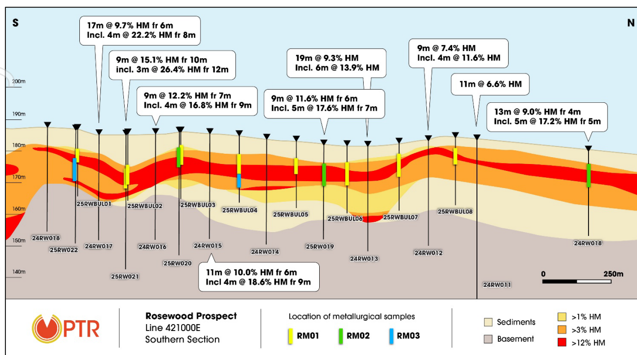
Figure 2: Rosewood East cross section – location of metallurgical composites and significant intercepts from historical exploration drilling¹.
