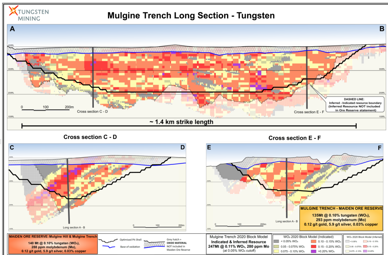
Figure 9: Mulgine Trench Long and Cross Sections 11
