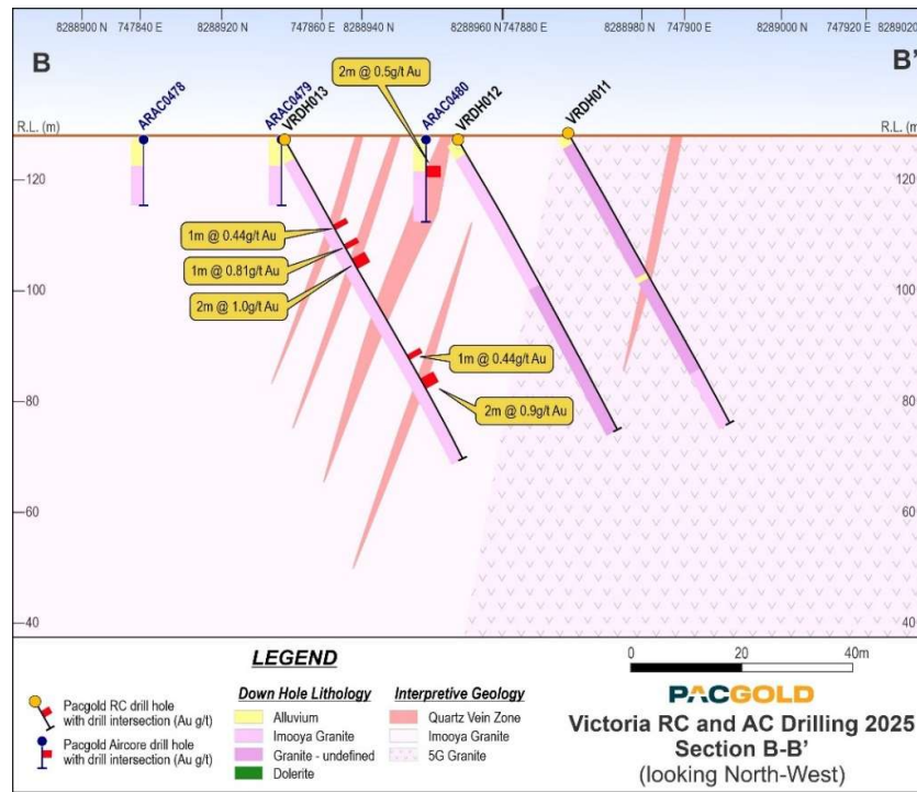
Figure 6: Victoria RC Drilling section B – B' (refer to Figure 4 for section location).
