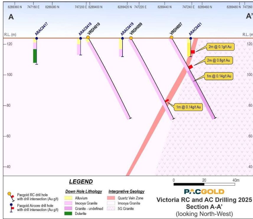
Figure 5: Victoria RC Drilling section A – A' (refer to Figure 4 for section location).
