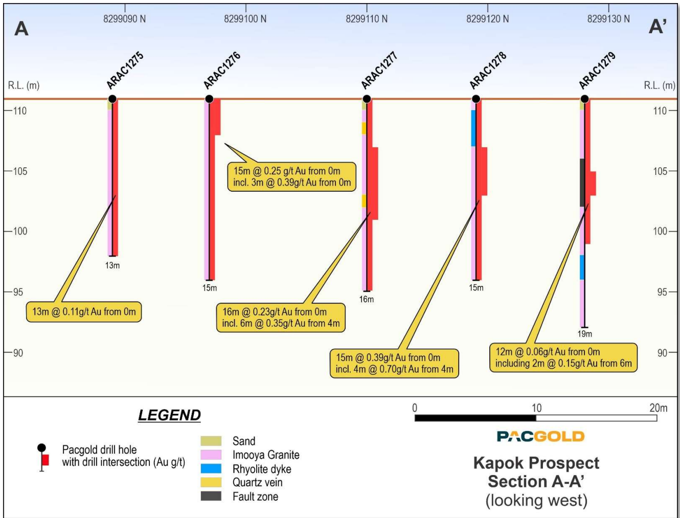
Figure 3: First pass Kapok aircore drill fence completed to test previously mapped and sampled quartz vein subcrop and float.
