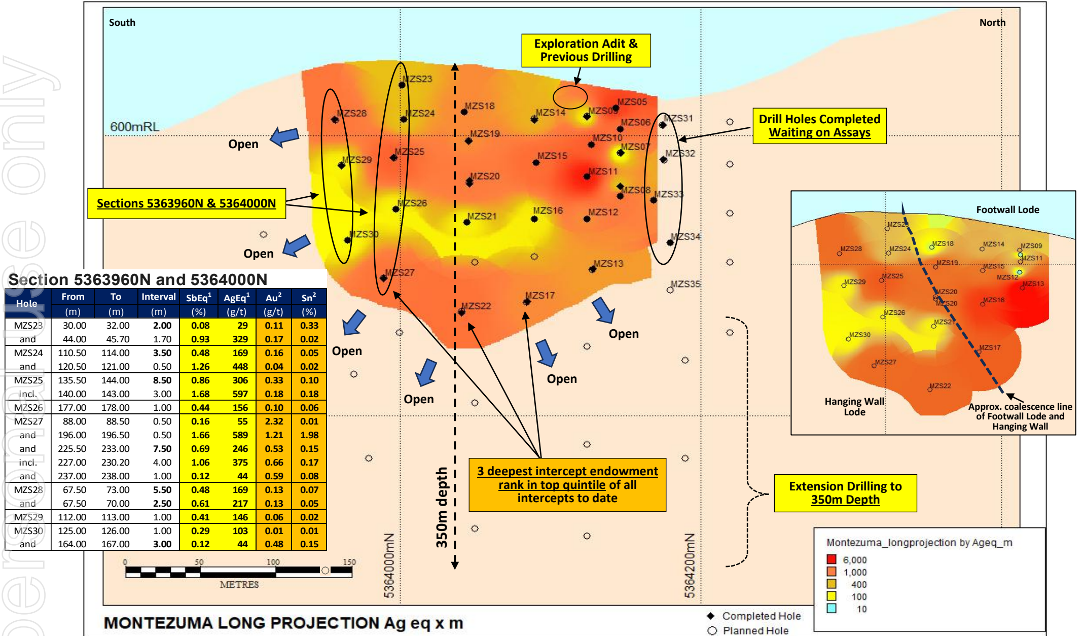
Figure 1. Montezuma Silver & Antimony Hanging Wall Lode Long Section SbEq 1 & AgEq 1 intercepts plus Au 2 and Sn 2 intercepts in drill holes MZS23 to MZS30 (5363960N & 5364000N)
