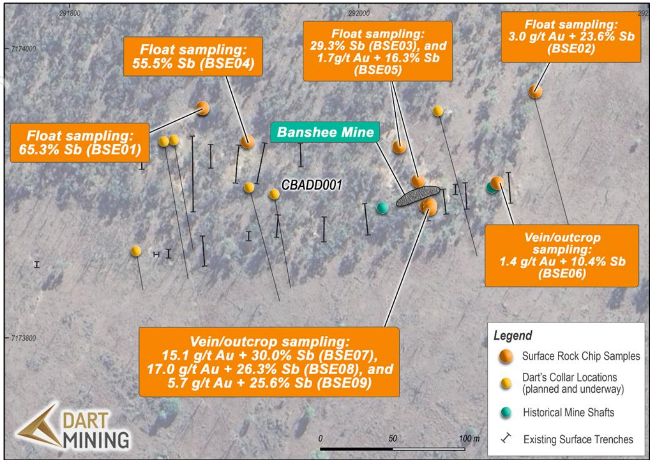
Figure 1 Location plan showing planned hole locations
