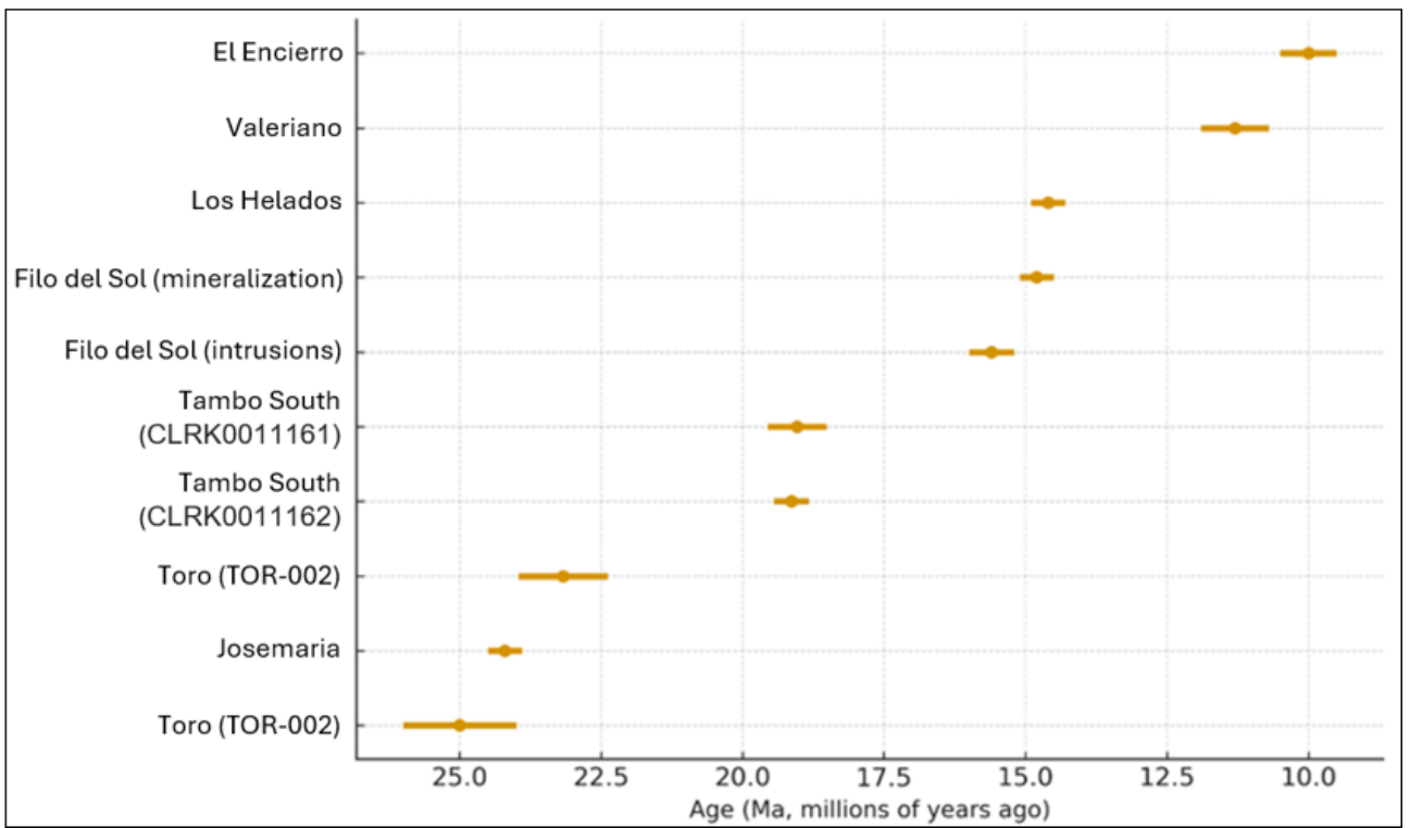
Figure 9: Interpreted magmatic ages from Toro and Tambo South compared with major Cu deposits nearby. Baseline deposit ages derived from Perello et al. (2023).
