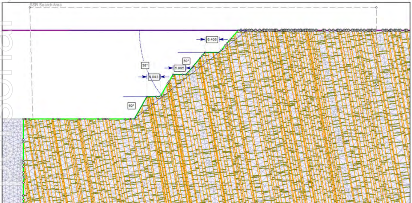
Figure 4.28 - Tested East Wall Geometry
