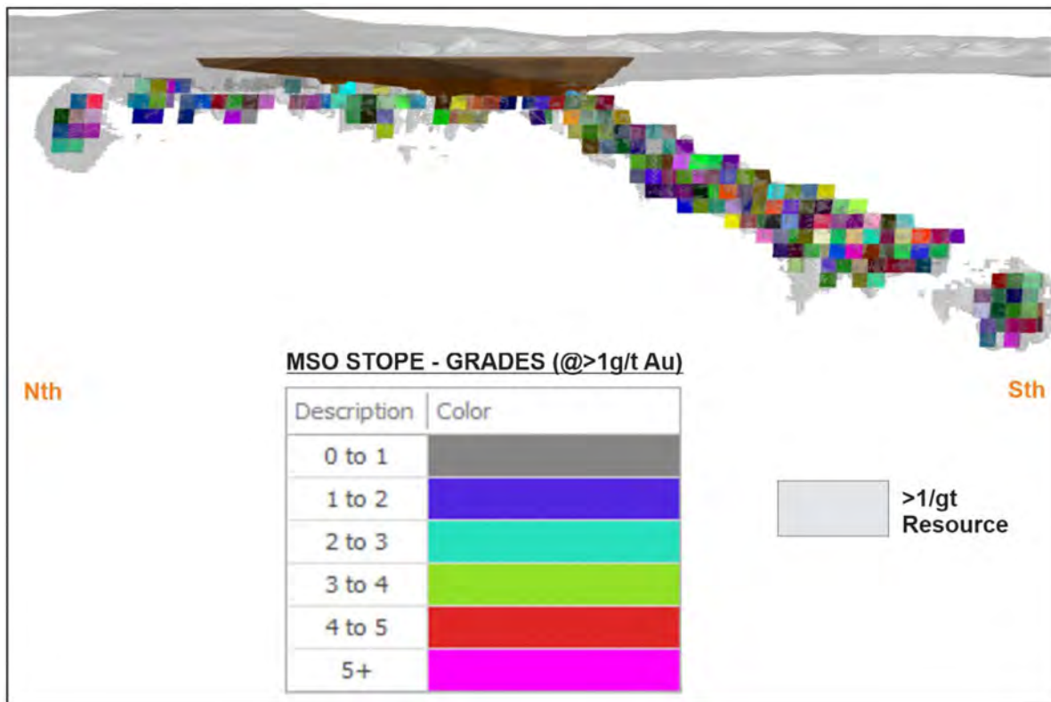
Figure 8.1 - Long Section Facing East Showing Generated MSO Stopes
