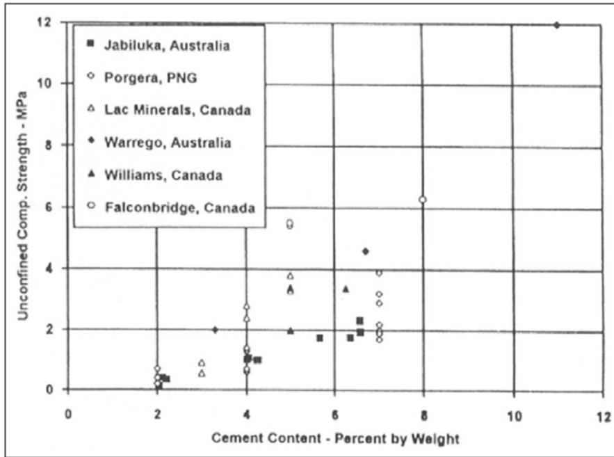
Figure 4.34 - UCS (500mm) for Various CRF Mixes Worldwide
