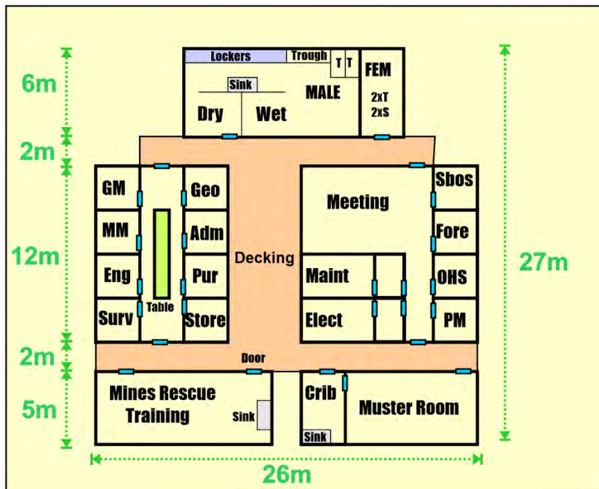
Figure 16.2 - Central Administration Facilities Conceptual Layout.
