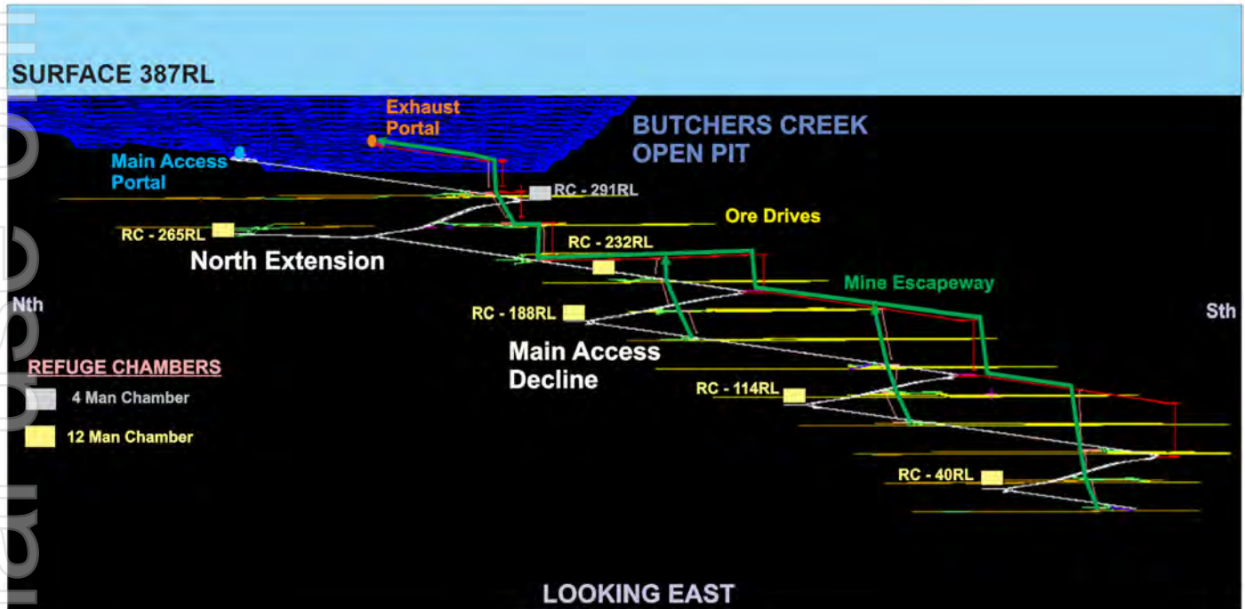
Figure 7.7 - Underground Escapeway System & Refuge Chambers
