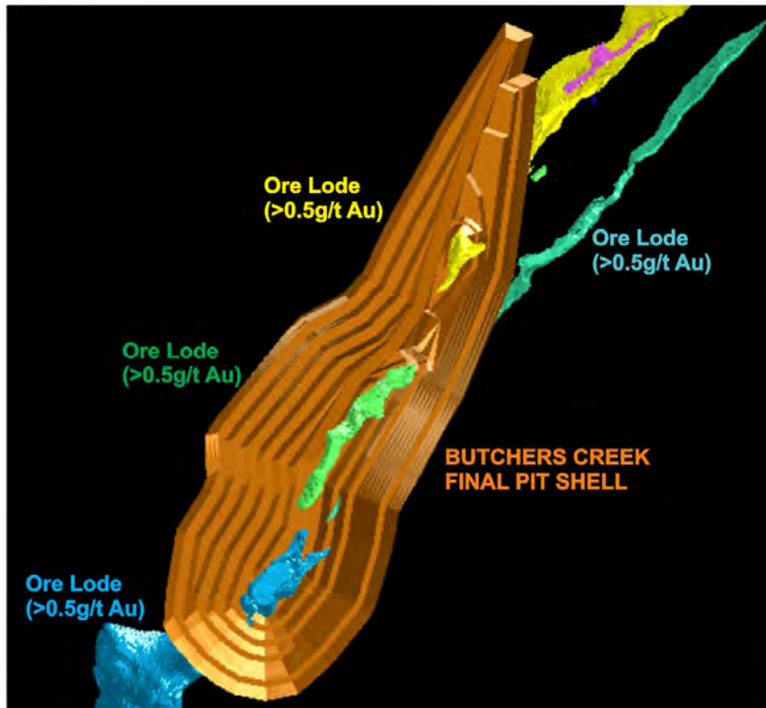
Figure 5.1 - Plan View of Butchers Creek Open Pit Design
