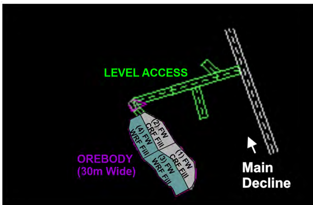
Figure 6.10 - Double Pass BU Long Hole Stoping with CRF & WRF (DPBULHS)
