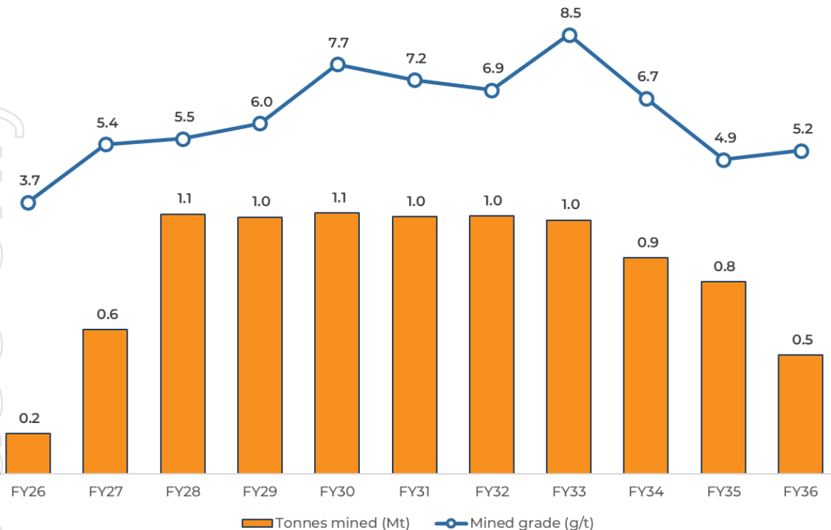
NEVER NEVER MINING SCHEDULE (Mt) & (g/t)
