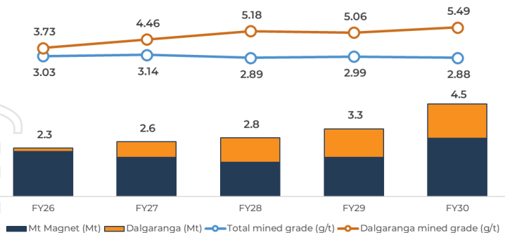
ORE MINING SCHEDULE (Mt) & (g/t)
