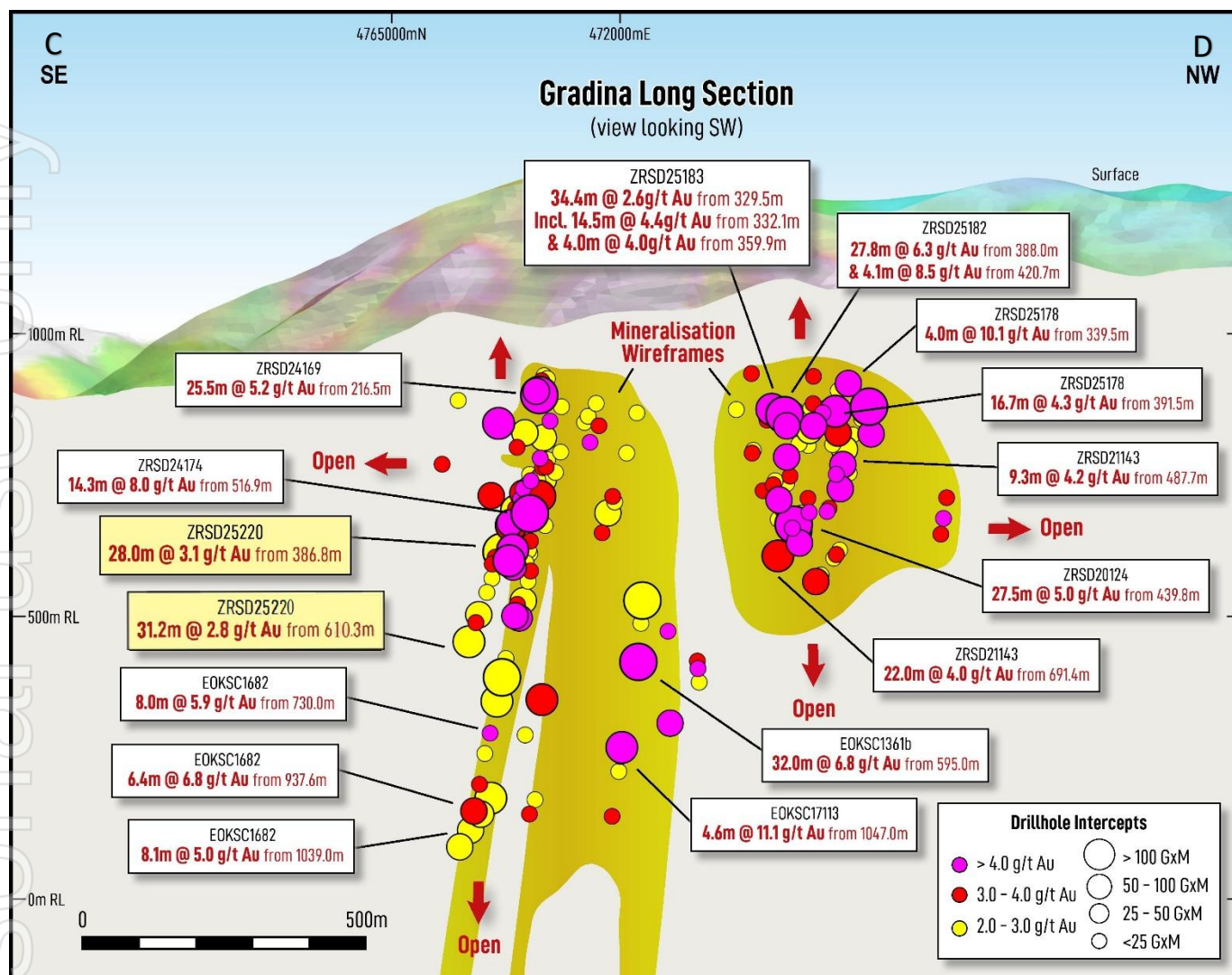
Figure 4. Gradina long-section view along C-D, showing results for ZRSD25212 and ZRSD25220 in relation to previously reported high-grade drill intercepts.
