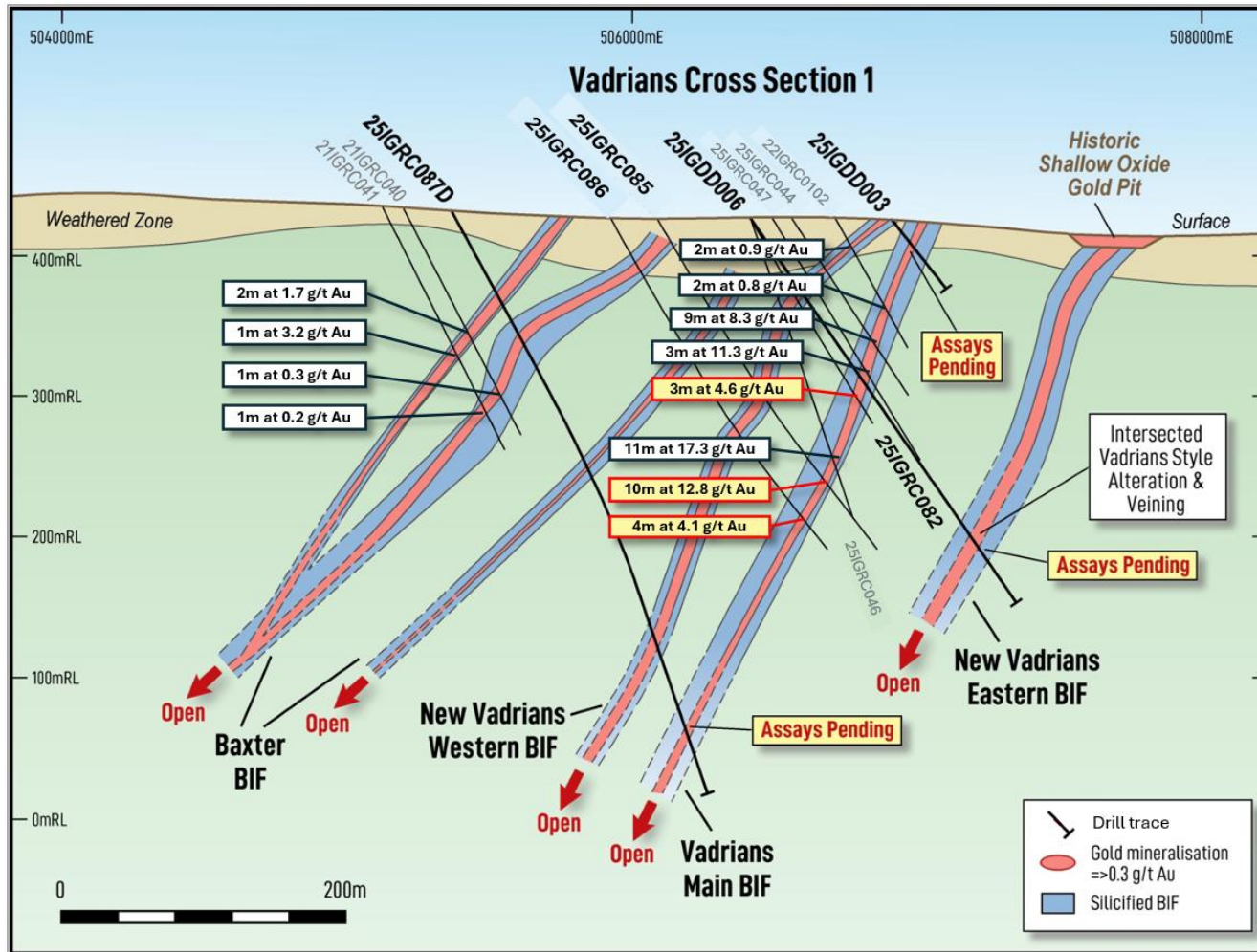
Figure 4. Vadrians Cross Section 1 (6942800mN): Highlighting the vertical depth extension from ~200m to ~400m pending assay results. The section also highlights additional stacked Banded Iron Formation (BIF) to the west with the potential for stacking and mineralisation to the East. Cross section window ± 50m.
