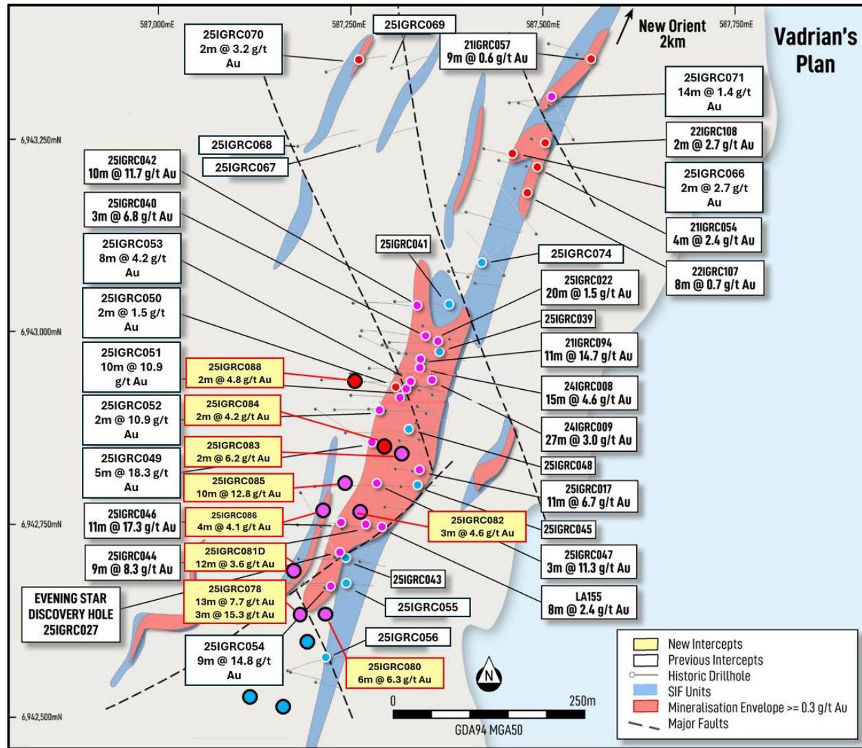
Figure 3: Plan of the Vadrians gold mineralisation with recently received significant assays.
