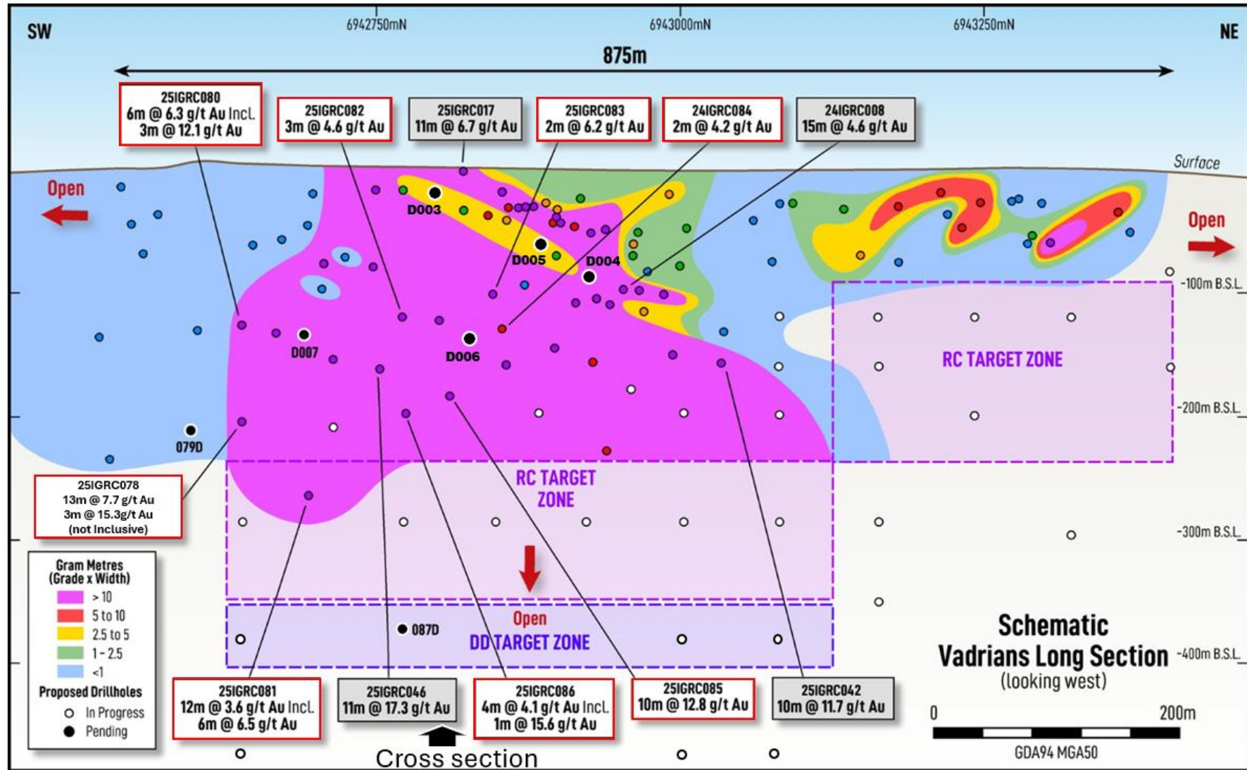
Figure 2: Schematic long section of the Vadrians gold mineralisation with recently received significant assays.
