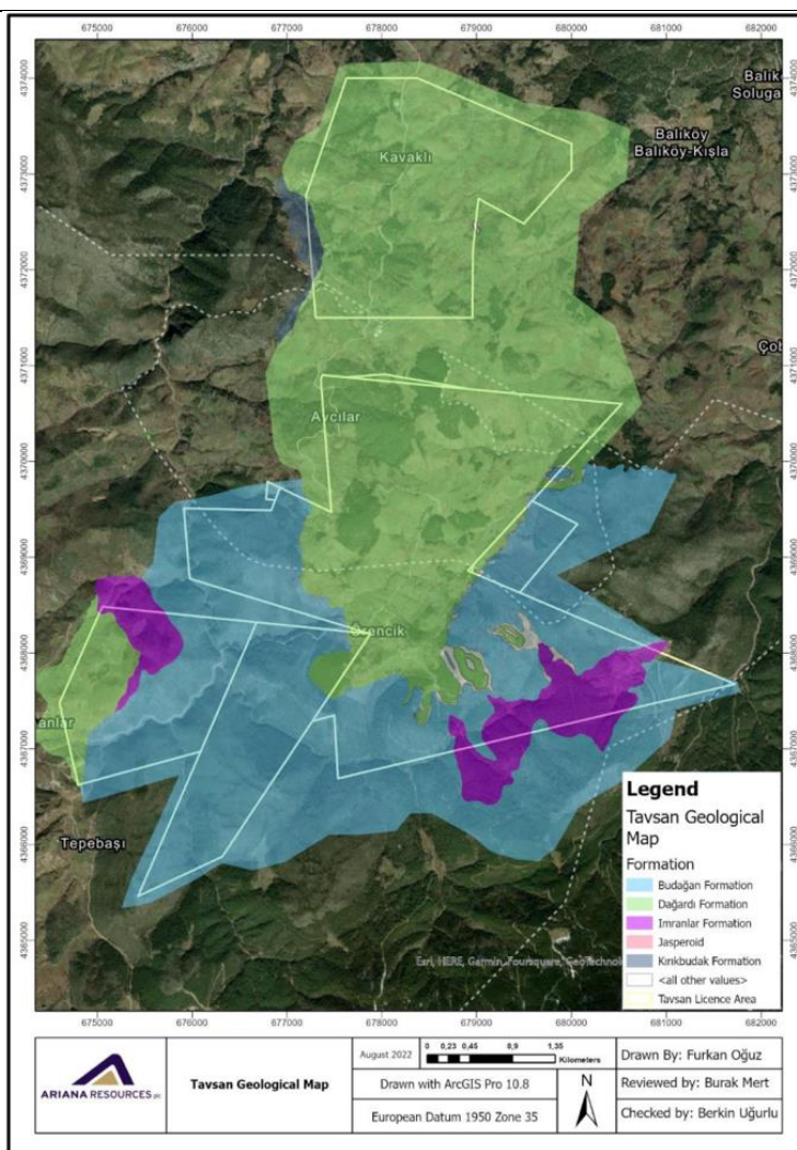
Figure 12. Tavsan Geological Map shows formations.
