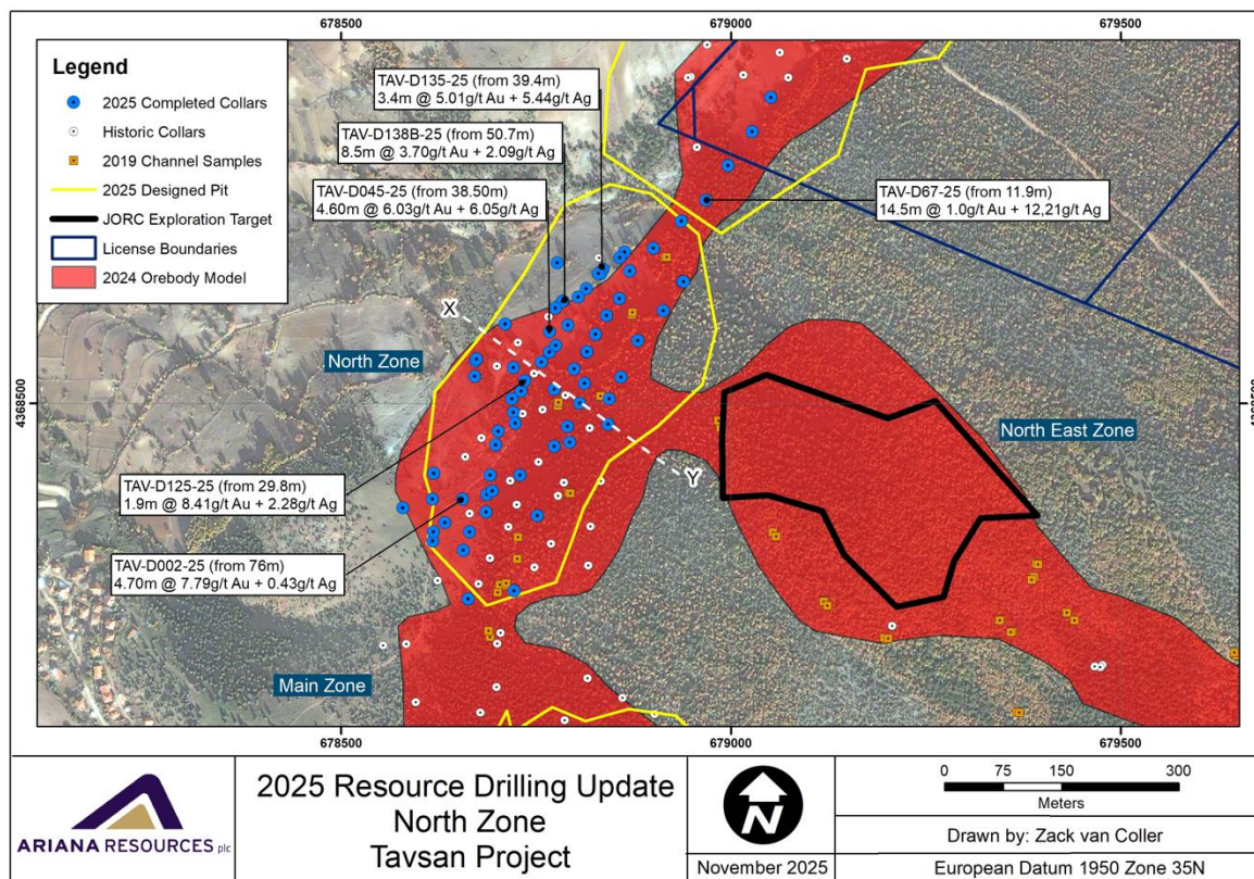
Figure 1: Plan view of Tavsan showing historic and recently completed drilling in the North Zone in relation to the currently defined resources, currently planned pit outlines and target areas.
