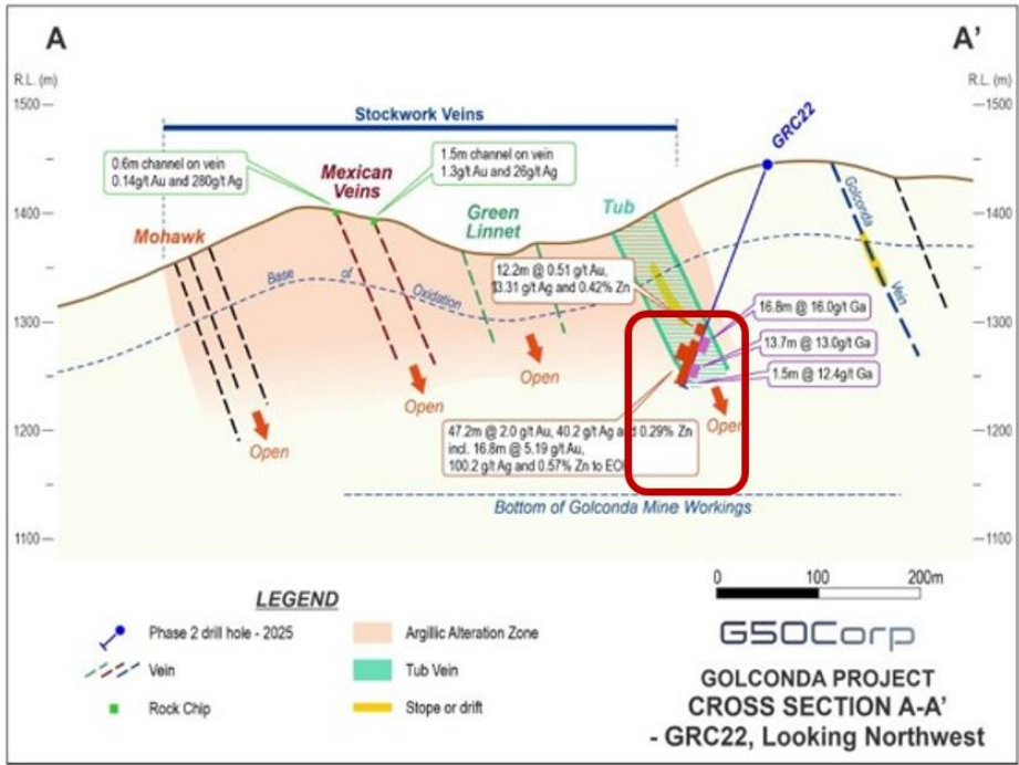
Figure 3 - Golconda Core drilling target in RED. Shown on Cross section A - A' relative to 2025 discovery hole GRC 22 - 47.2m at 2.0g/t gold, 40.2g/t silver and 0.29% zinc, from 191 meters to EOH.
