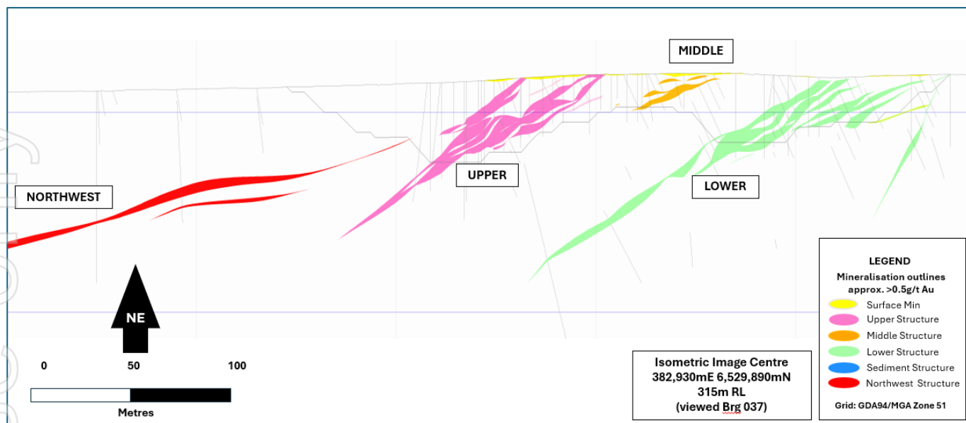
Figure 5: Geological long section looking towards the north-east showing Upper Structure, Middle, Lower and NWP Structures - a slice through a potential open pit shell.
