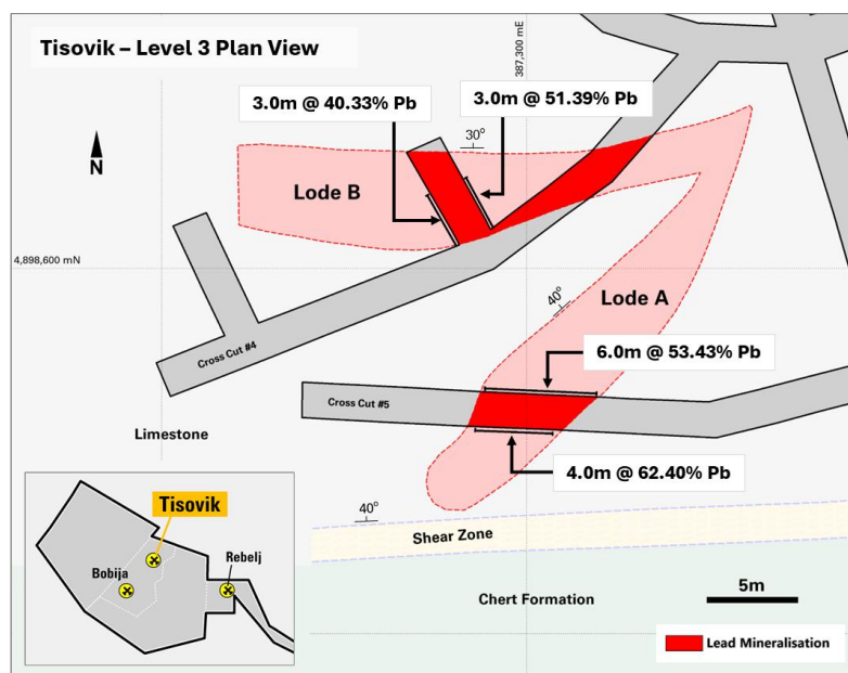
Figure 5: Tisovik Mine - Plan view of Level 3 workings showing composite historic lead face sample results (refer to Table 1 for details of individual sample intervals). (1)
