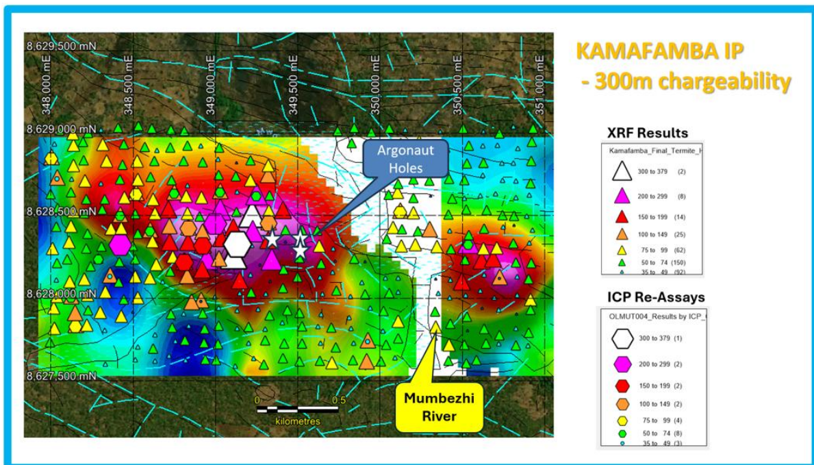
Figure 5: Kamafamba Prospect – showing termite hill copper geochemistry over chargeable IP data and historical Argonaut Resources drill holes (combined AEM/geochemical anomaly is ~2km long)
