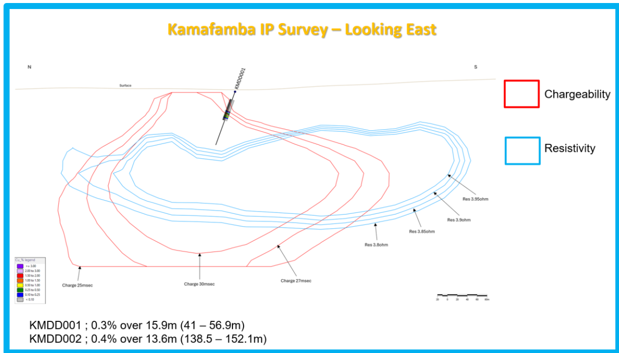
Figure 6: Kamafamba Prospect – long section (looking east) through overlapping chargeable and resistivity IP shells and historical drill hole KMDD001 (drilled too short)
