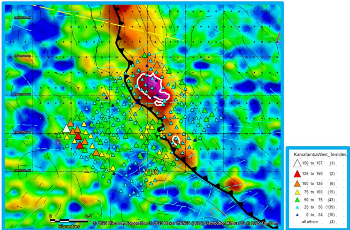
Figure 7: Kamafamba West Prospect – Termite hill geochemical copper results displayed over AEM imagery open to northwest on interpreted fault/thrust structures
