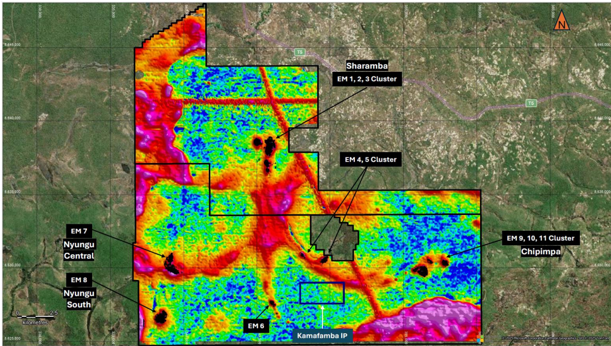
Figure 1: Mumbesghi Project – Licence wide processed EM geophysical output showing identified strong EM conductors and prospect locations
