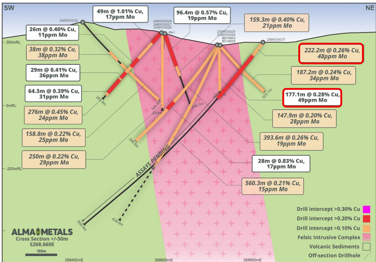
Figure 2. Cross Section showing down-hole geology in 25BRD0037 and the assays for the top 231m of the hole (red label outlines). For location refer to Figure 1.
