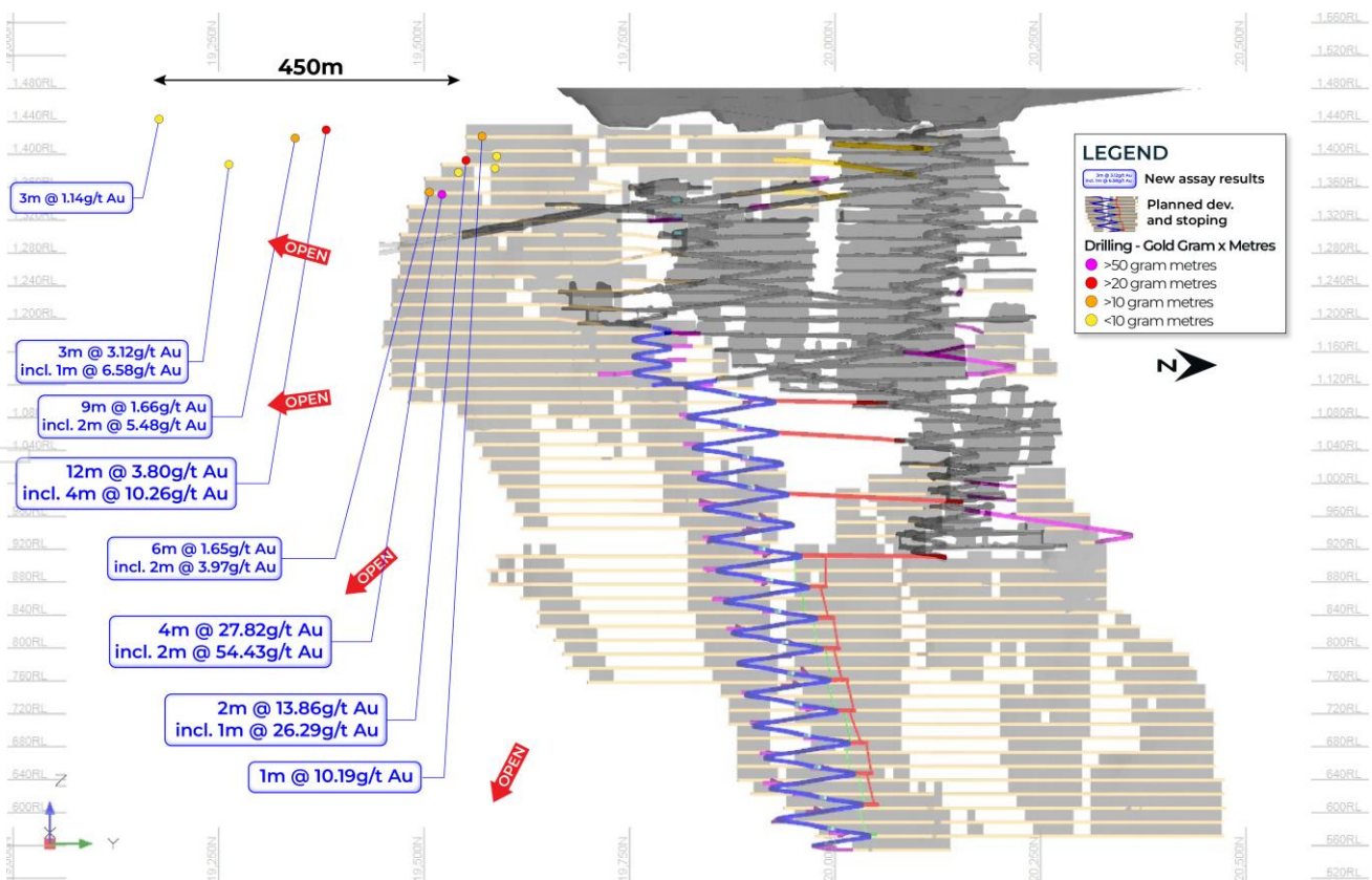
Figure 2: Long section showing new high-grade Resource extension drilling results and life of mine development and stopping on the Wilber lode at Andy Well.
