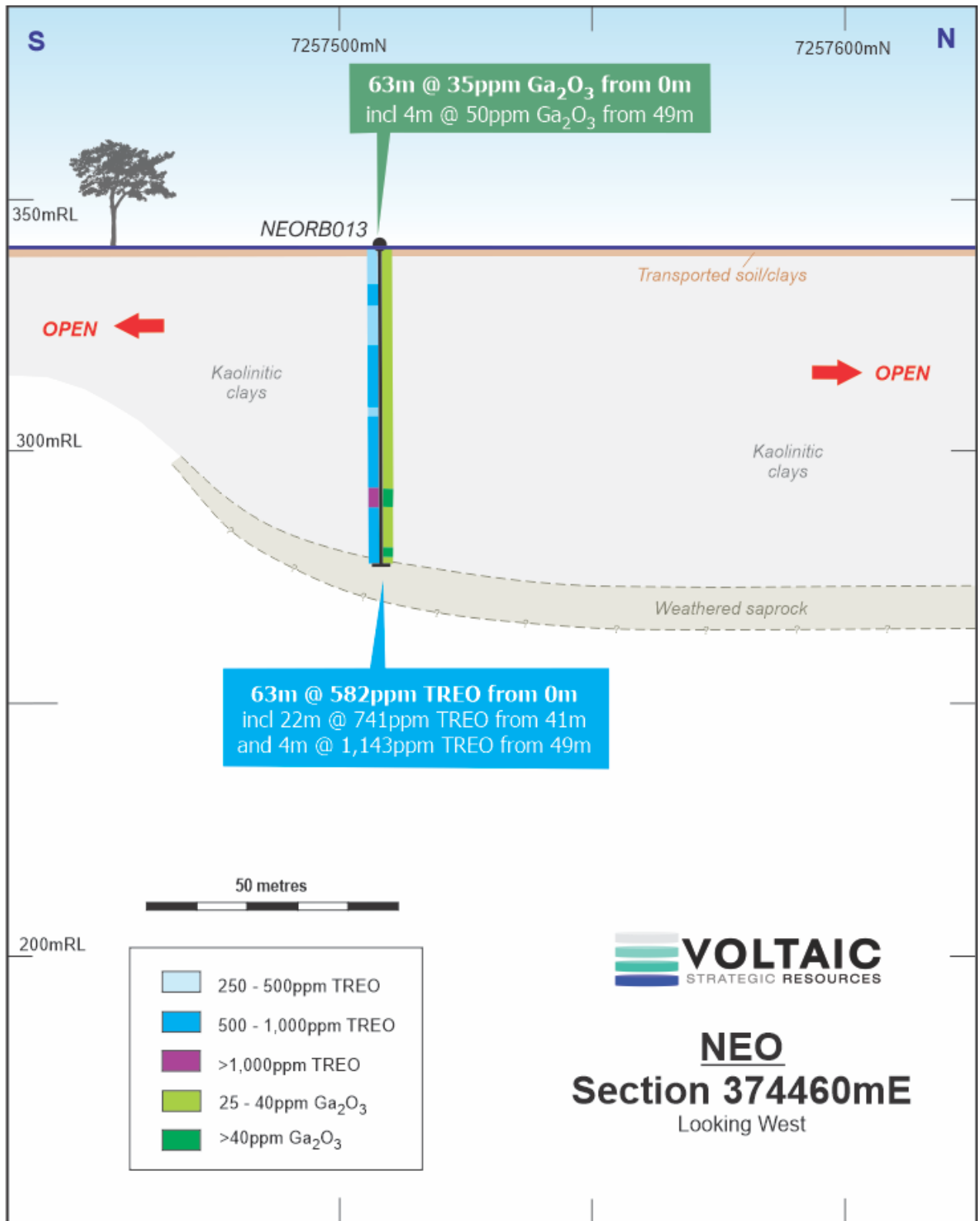
Figure 9. Neo MREO-Ga mineralised system – Section 374460E
