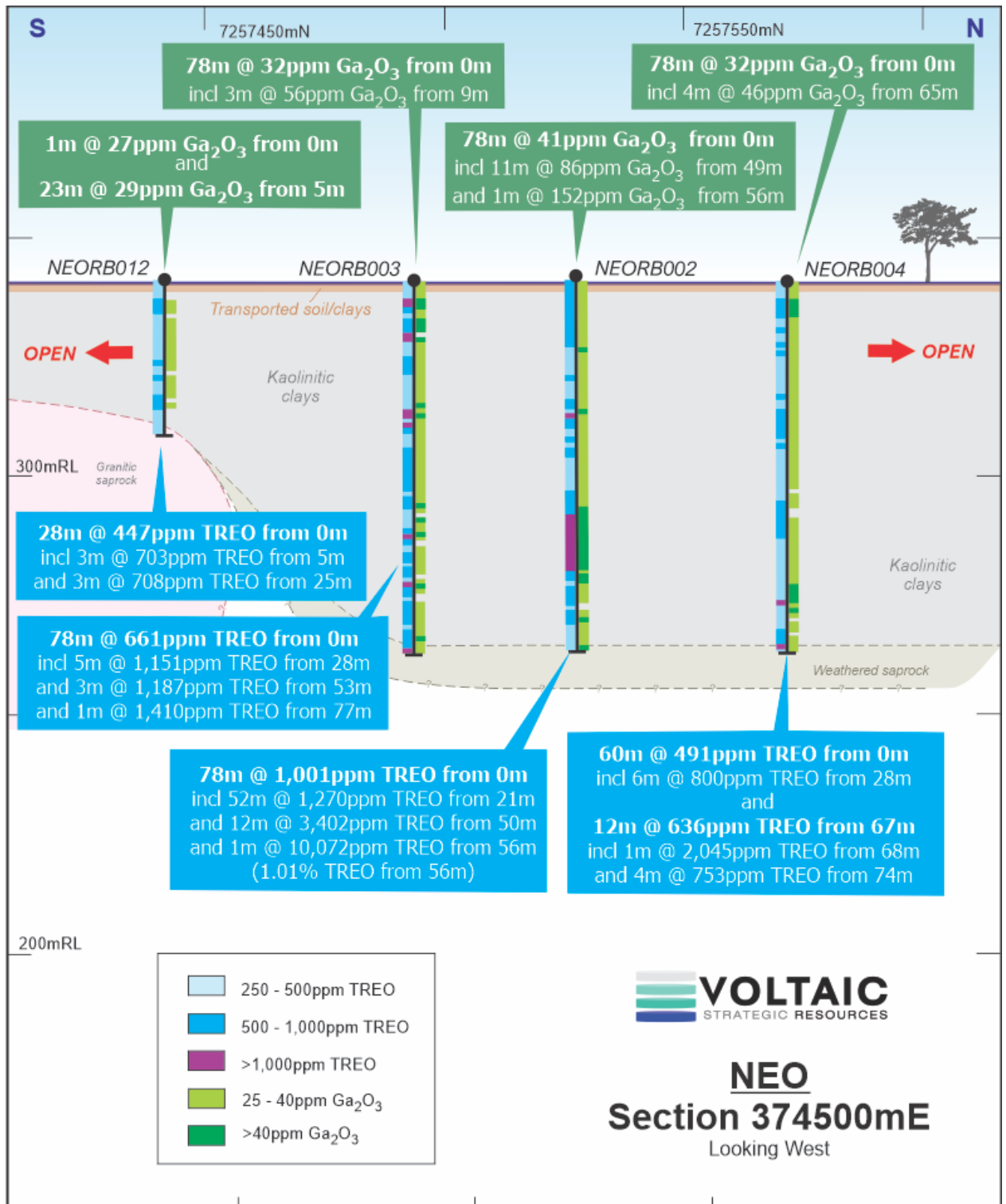
Figure 8. Neo MREO-Ga mineralised system – Section 374500E
