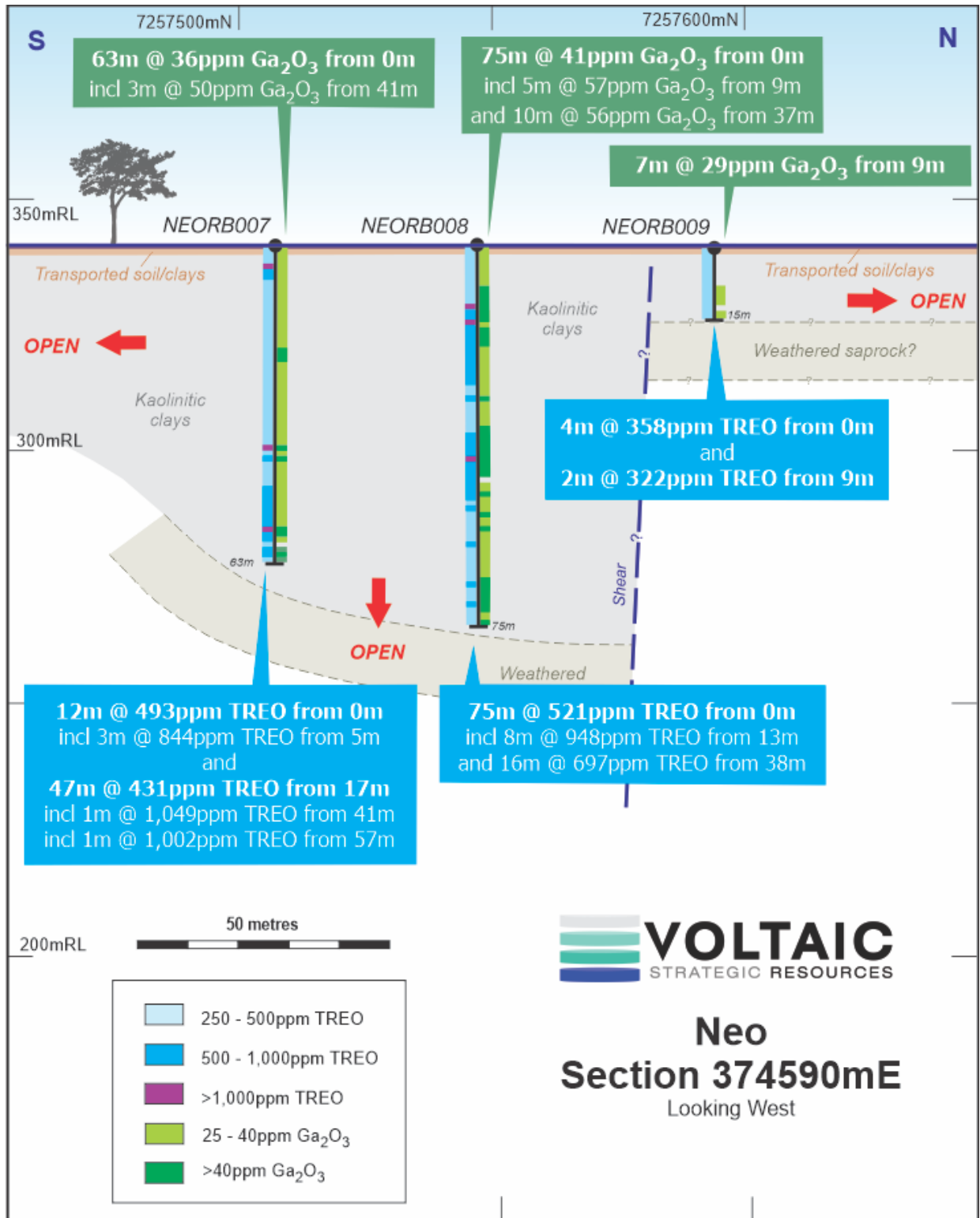
Figure 7. Neo MREO-Ga mineralised system – Section 374590E
