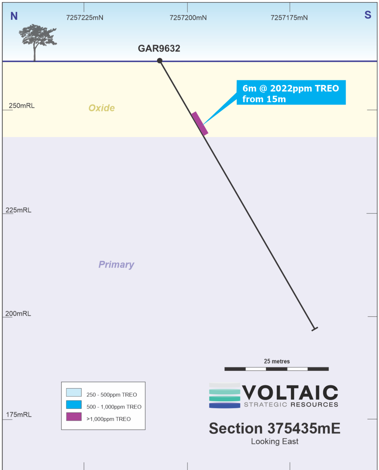
Figure 12. Link MREO mineralised system – Section 375435E
