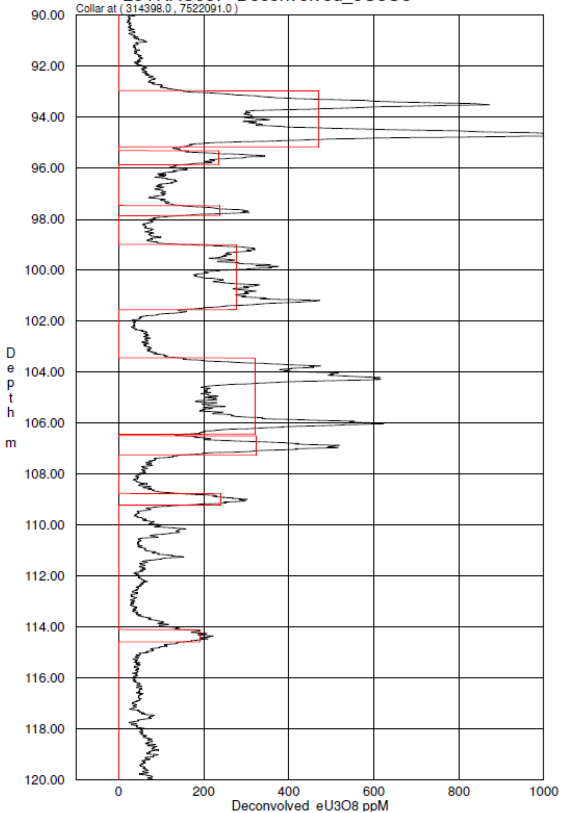
Figure 6. 25YRAC037 deconvolved downhole gamma log showing mineralised intervals detailed in Table 2.
