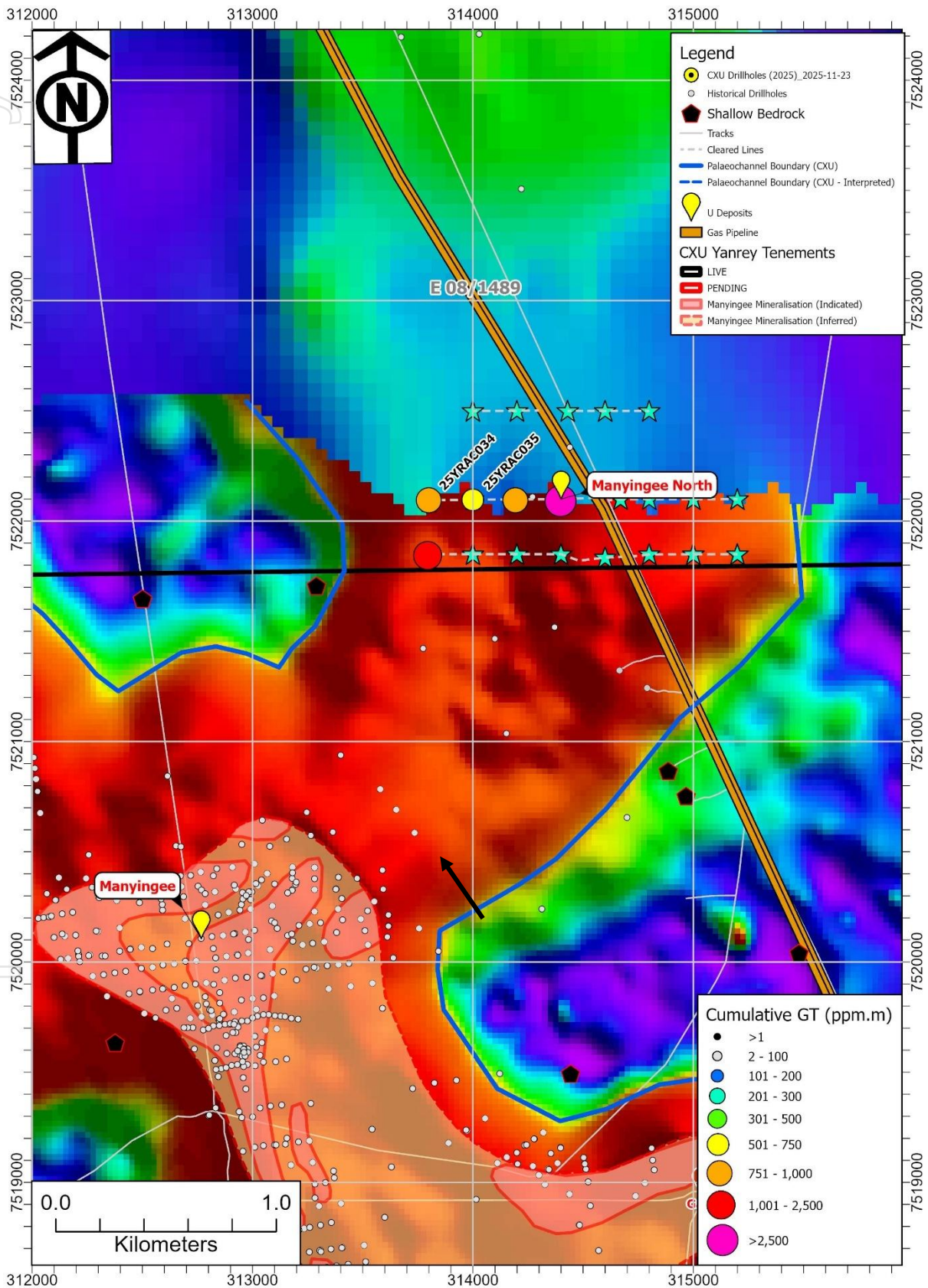
Figure 5. Manyingee North combined RepTEM (southern half) and HeliTEM (northern half) geophysical imagery showing the location of the Manyingee North palaeochannel in relation to mineralisation defined at Manyingee. Note that the two TEM surveys have different colour schemes. Mineralisation at Manyingee continues to the northwest having apparently been closed off by the line of 4 holes (black arrow) whilst the Manyingee North palaeochannel is largely unexplored.
