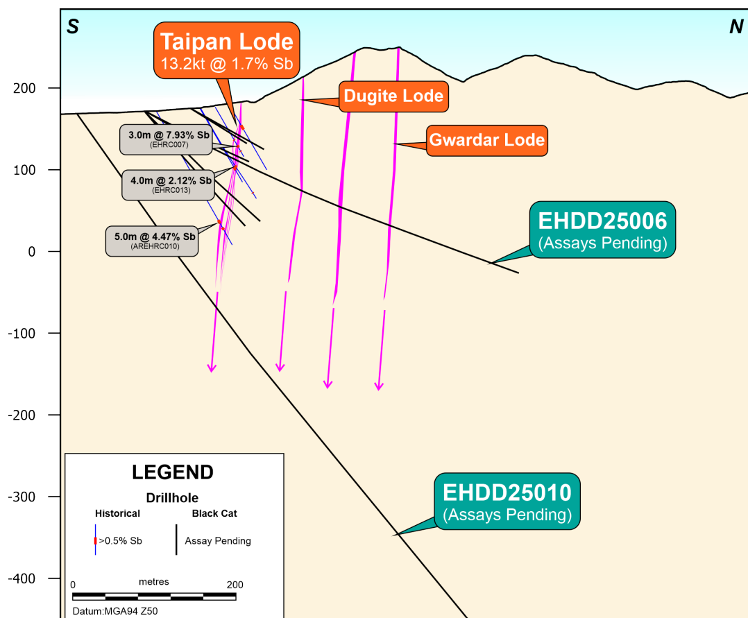
Figure 5: Cross-section looking west showing current exploration drillholes EHDD25006 and EHDD25010, that intersected additional antimony lodges to the north of the Taipan Lodge. Assays are pending for both holes. Historical drill results are shown from within the Taipan Lodge 7
