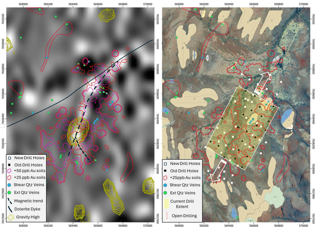
Figure 2. LHS. Drill holes showing magnetic and gravity trends with Au in soils and mapped quartz veins RHS. Drill holes showing satellite mage with geological map, Au in soils and mapped quartz veins
