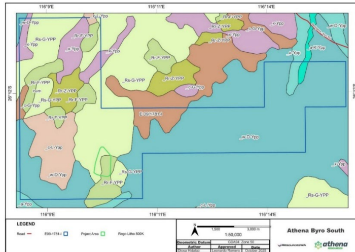
Figure 5: Byro Project Local Geology
