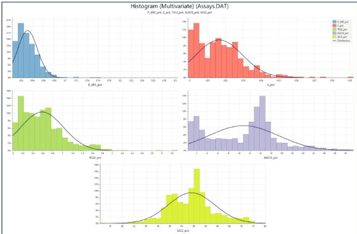
Figure 6: Byro South Minor Element Distributions
