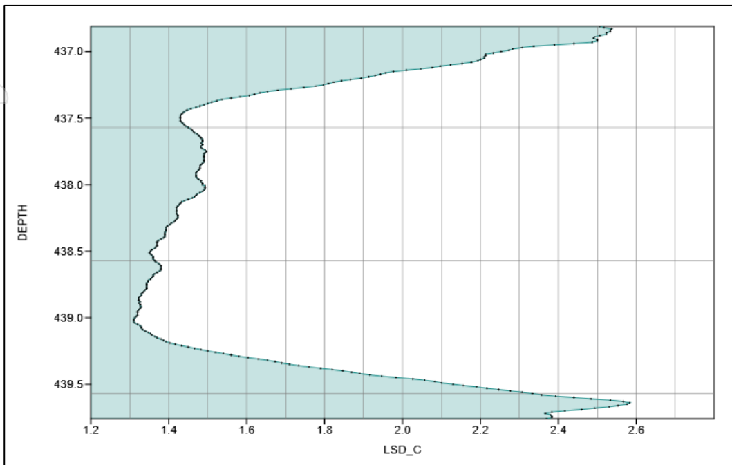
FIGURE 5: RSC015C - "B" AND "D" SEAM LONG-SPACED DENSITY PROFILES
