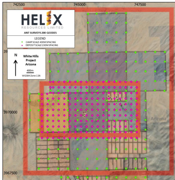
Figure 1. Passive seismic station layout across the White Hills Project area showing camp-scale (400 m) and deposit-scale (230 m) ANT spacing (Fleet ANT Proposal 2025).
